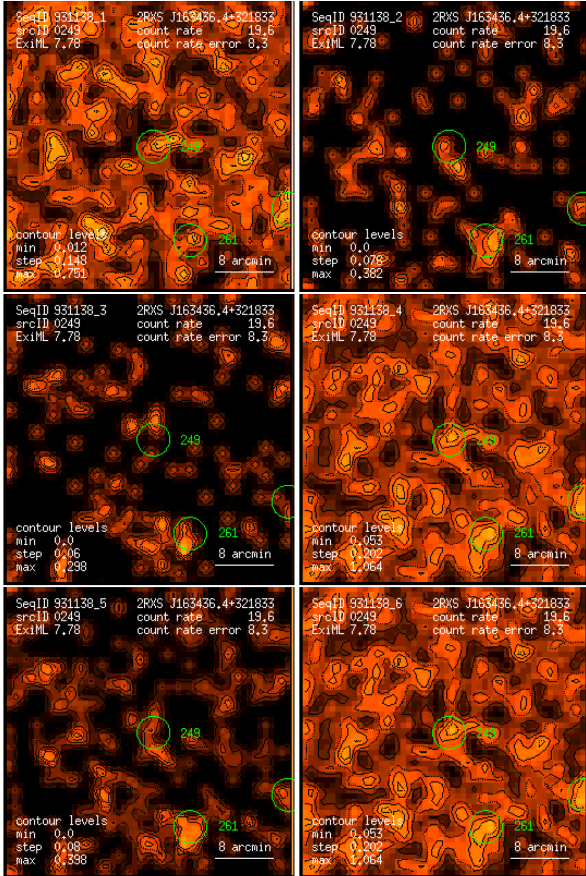
Figure 249: RASS 931138: detection 0249: band rate images, Gaussian filter: (1) PSPC channels 11 – 41, (2) 52 – 90, (3) 91 – 201, (4) 11 – 235, (5) 52 – 201, (6) 11 – 201. Broad band rates in counts/ks. Band rate contour levels in counts/ks/arcmin 2 .
