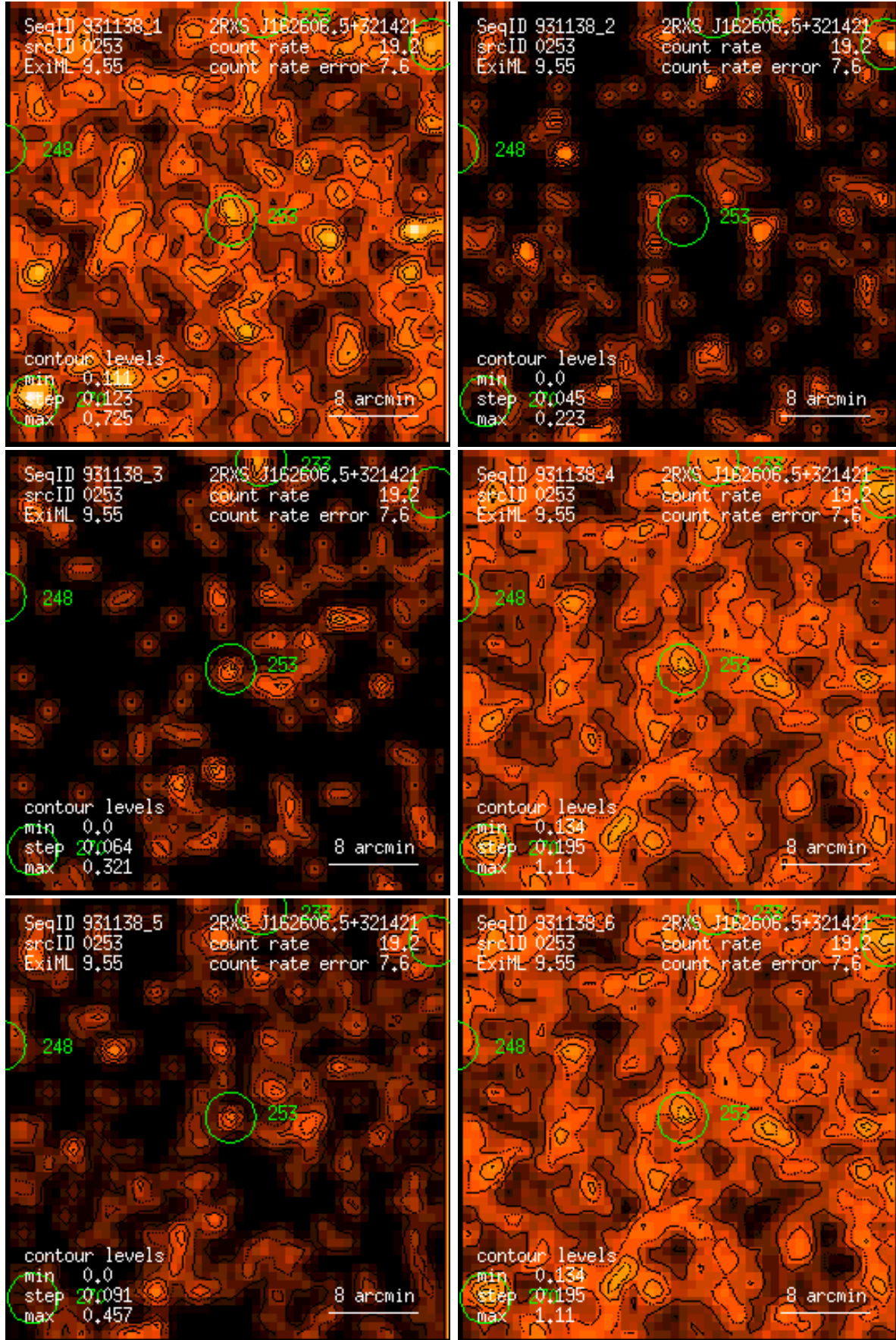
Figure 253: RASS 931138: detection 0253: band rate images, Gaussian filter: (1) PSPC channels 11 – 41, (2) 52 – 90, (3) 91 – 201, (4) 11 – 235, (5) 52 – 201, (6) 11 – 201. Broad band rates in counts/ks. Band rate contour levels in counts/ks/arcmin 2 .
