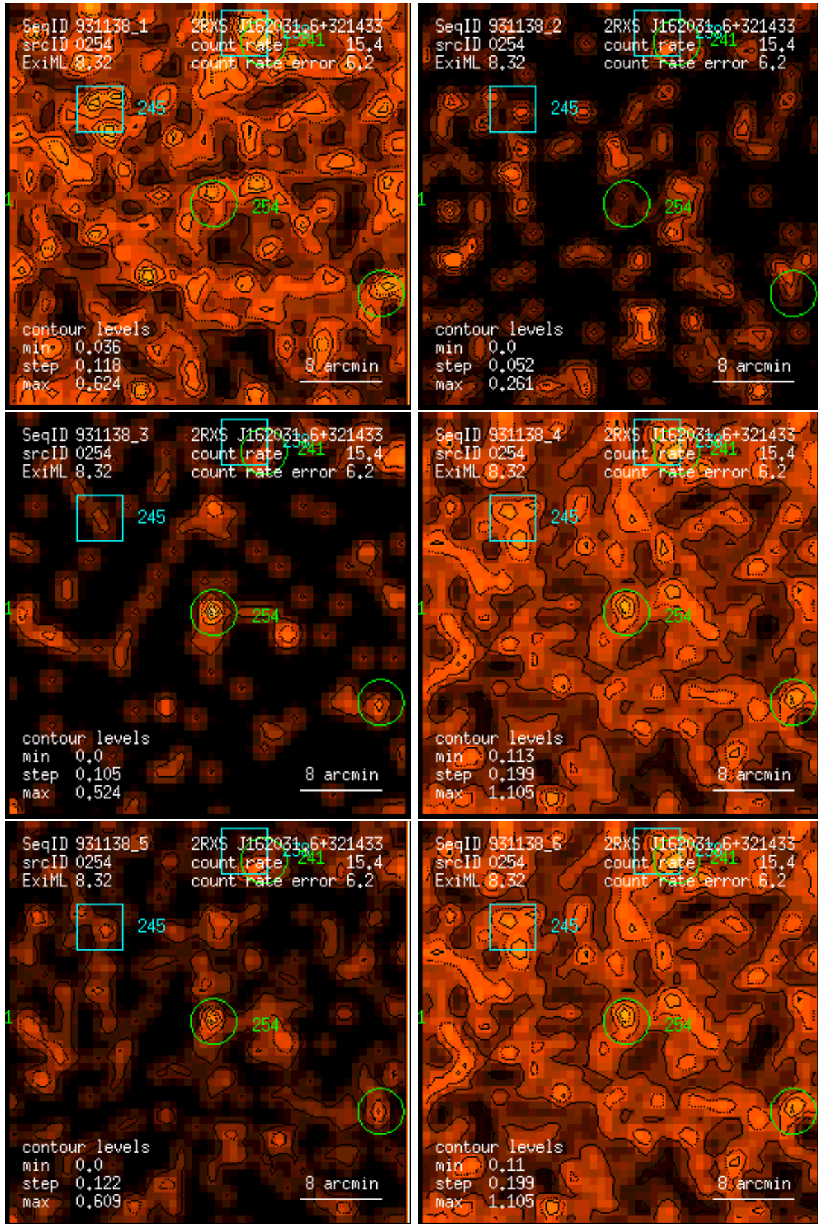
Figure 254: RASS 931138: detection 0254: band rate images, Gaussian filter: (1) PSPC channels 11 – 41, (2) 52 – 90, (3) 91 – 201, (4) 11 – 235, (5) 52 – 201, (6) 11 – 201. Broad band rates in counts/ks. Band rate contour levels in counts/ks/arcmin 2 .
