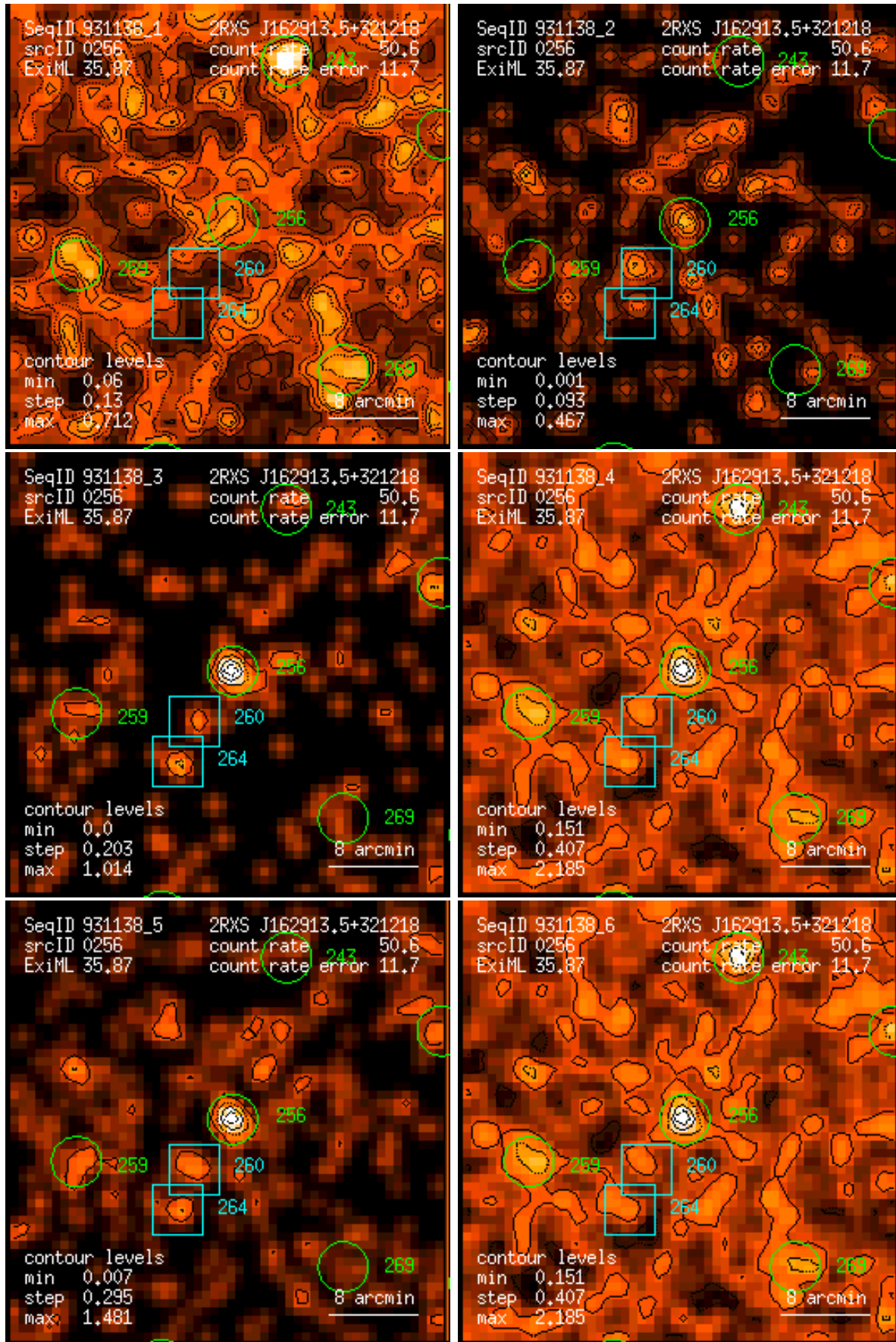
Figure 256: RASS 931138: detection 0256: band rate images, Gaussian filter: (1) PSPC channels 11 – 41, (2) 52 – 90, (3) 91 – 201, (4) 11 – 235, (5) 52 – 201, (6) 11 – 201. Broad band rates in counts/ks. Band rate contour levels in counts/ks/arcmin 2 .
