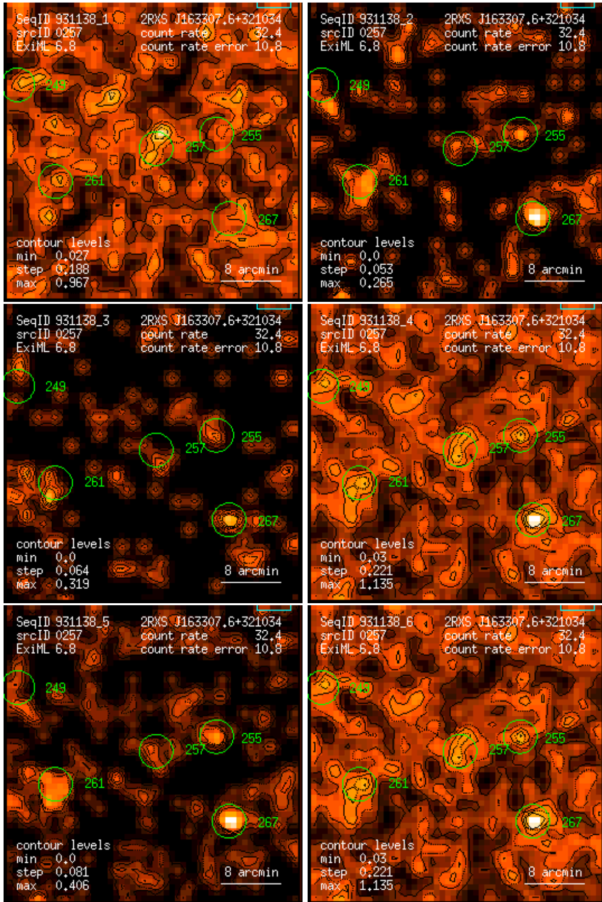
Figure 257: RASS 931138: detection 0257: band rate images, Gaussian filter: (1) PSPC channels 11 – 41, (2) 52 – 90, (3) 91 – 201, (4) 11 – 235, (5) 52 – 201, (6) 11 – 201. Broad band rates in counts/ks. Band rate contour levels in counts/ks/arcmin 2 .
