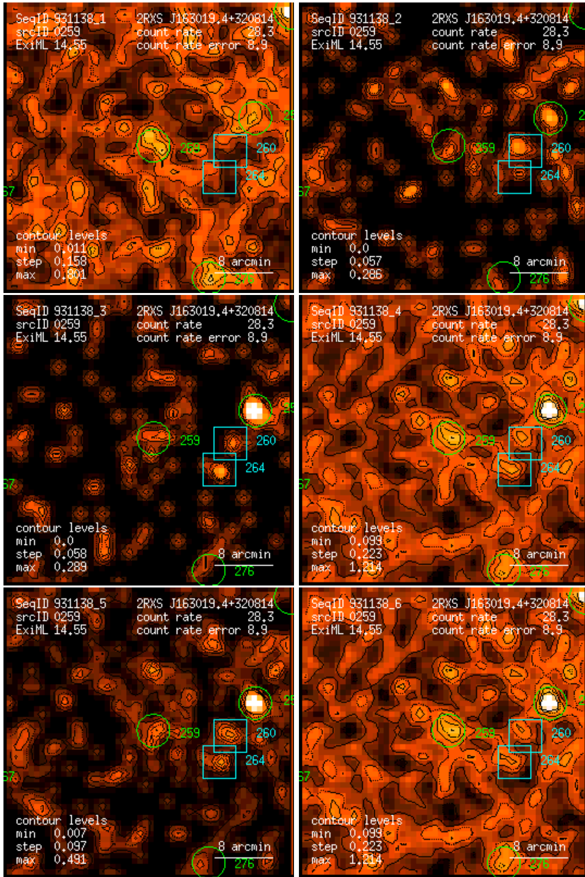
Figure 259: RASS 931138: detection 0259: band rate images, Gaussian filter: (1) PSPC channels 11 – 41, (2) 52 – 90, (3) 91 – 201, (4) 11 – 235, (5) 52 – 201, (6) 11 – 201. Broad band rates in counts/ks. Band rate contour levels in counts/ks/arcmin 2 .
