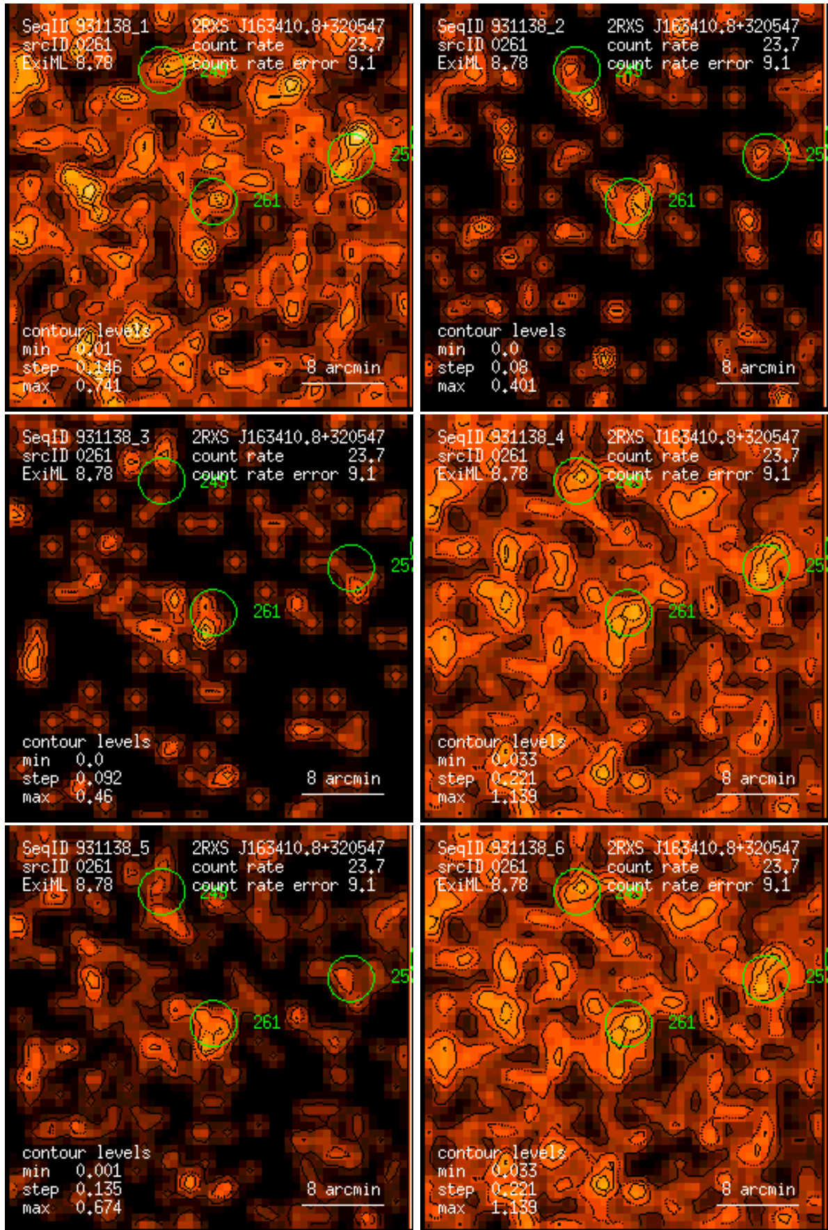
Figure 261: RASS 931138: detection 0261: band rate images, Gaussian filter: (1) PSPC channels 11 – 41, (2) 52 – 90, (3) 91 – 201, (4) 11 – 235, (5) 52 – 201, (6) 11 – 201. Broad band rates in counts/ks. Band rate contour levels in counts/ks/arcmin 2 .
