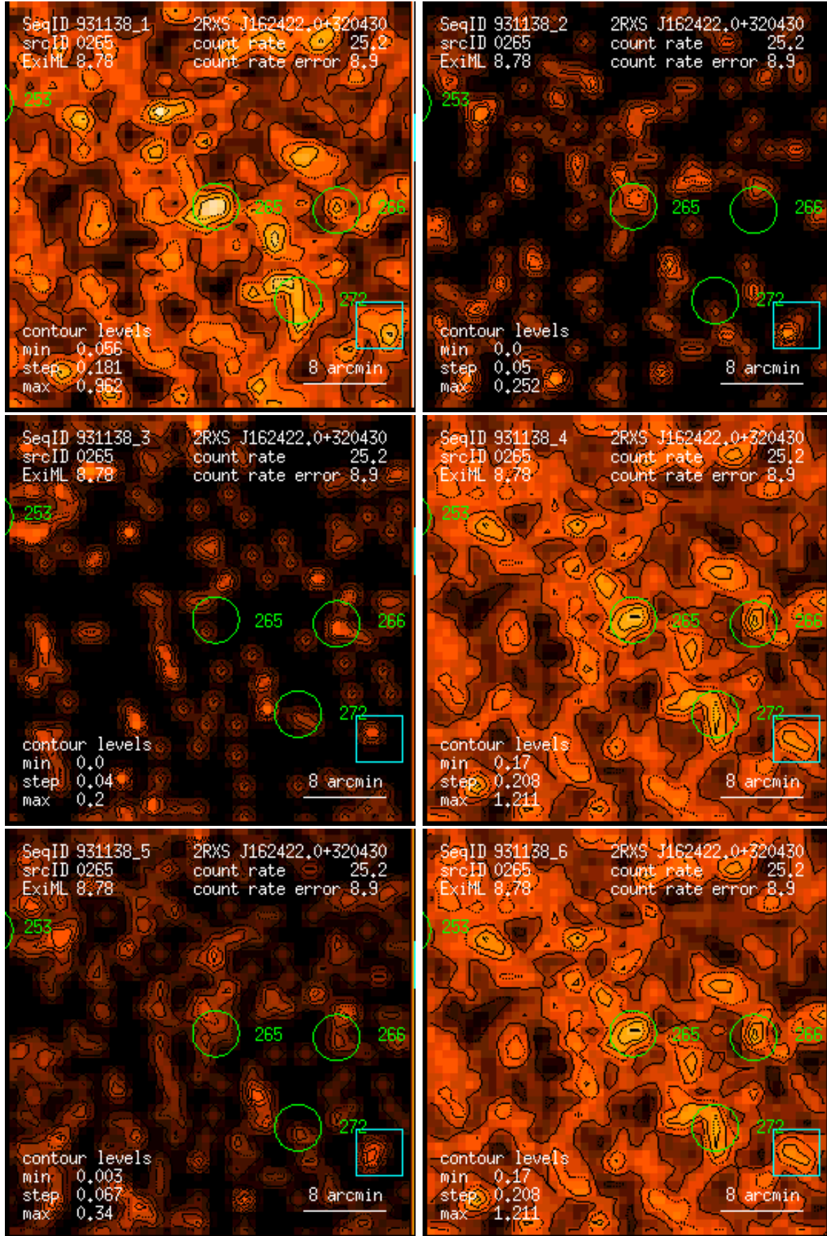
Figure 265: RASS 931138: detection 0265: band rate images, Gaussian filter: (1) PSPC channels 11 – 41, (2) 52 – 90, (3) 91 – 201, (4) 11 – 235, (5) 52 – 201, (6) 11 – 201. Broad band rates in counts/ks. Band rate contour levels in counts/ks/arcmin 2 .
