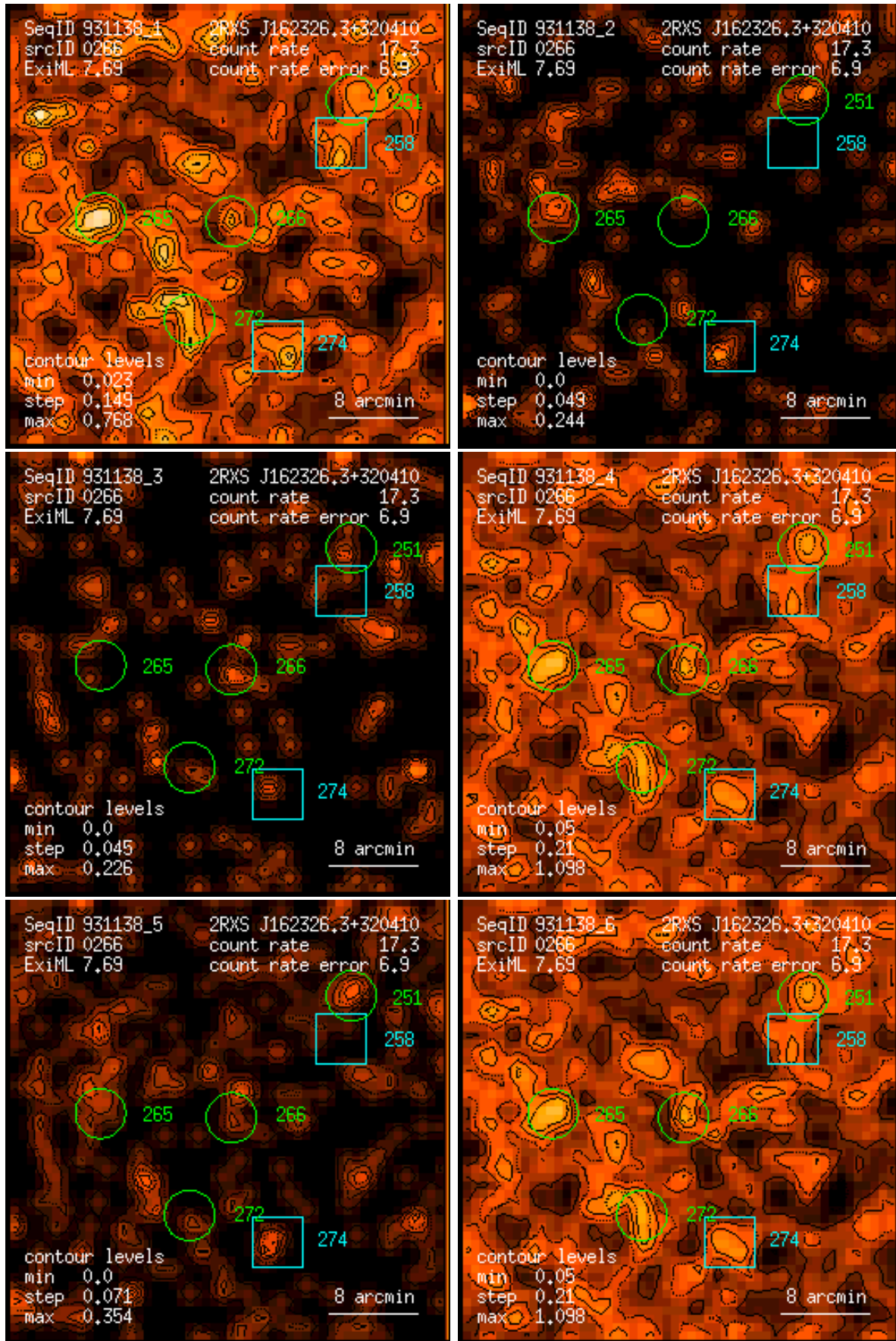
Figure 266: RASS 931138: detection 0266: band rate images, Gaussian filter: (1) PSPC channels 11 – 41, (2) 52 – 90, (3) 91 – 201, (4) 11 – 235, (5) 52 – 201, (6) 11 – 201. Broad band rates in counts/ks. Band rate contour levels in counts/ks/arcmin 2 .
