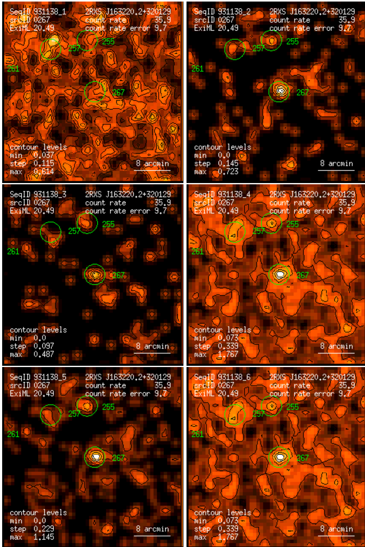
Figure 267: RASS 931138: detection 0267: band rate images, Gaussian filter: (1) PSPC channels 11 – 41, (2) 52 – 90, (3) 91 – 201, (4) 11 – 235, (5) 52 – 201, (6) 11 – 201. Broad band rates in counts/ks. Band rate contour levels in counts/ks/arcmin 2 .
