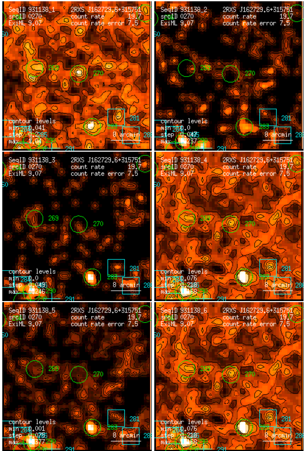
Figure 270: RASS 931138: detection 0270: band rate images, Gaussian filter: (1) PSPC channels 11 – 41, (2) 52 – 90, (3) 91 – 201, (4) 11 – 235, (5) 52 – 201, (6) 11 – 201. Broad band rates in counts/ks. Band rate contour levels in counts/ks/arcmin 2 .
