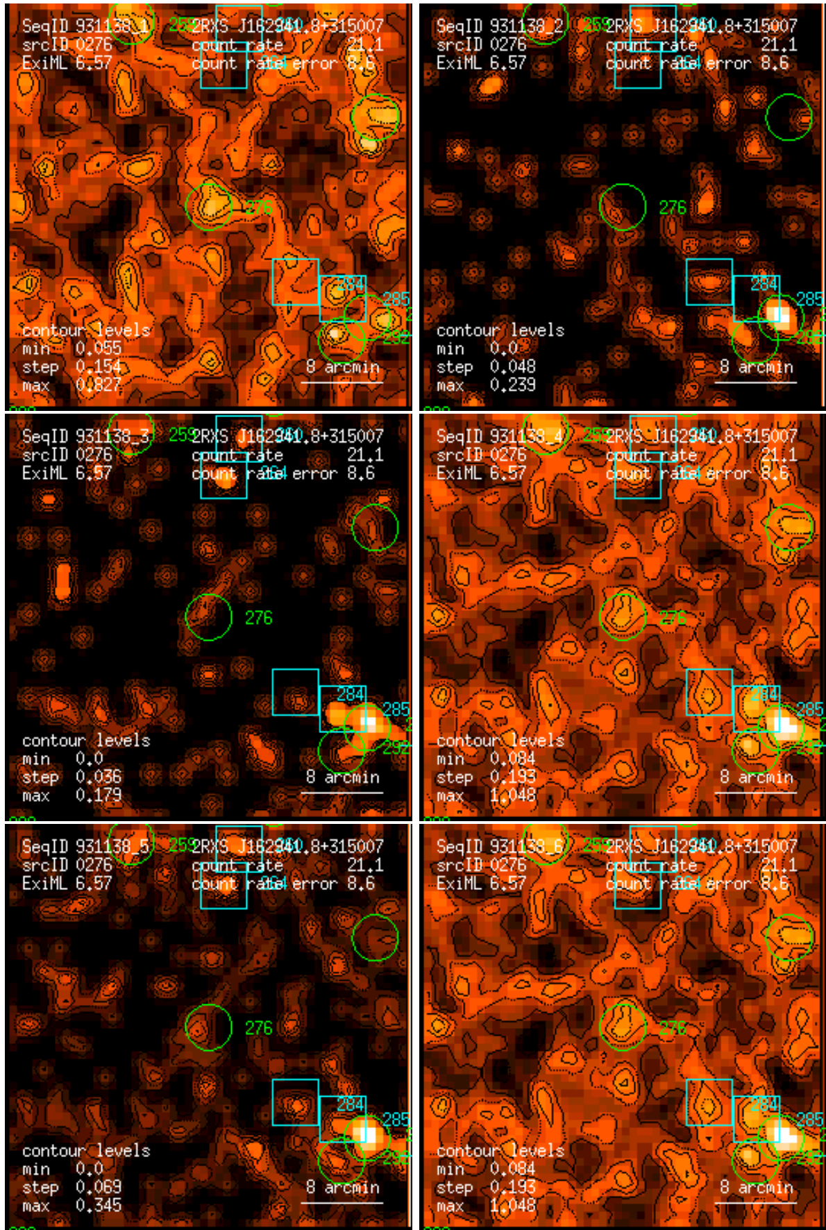
Figure 276: RASS 931138: detection 0276: band rate images, Gaussian filter: (1) PSPC channels 11 – 41, (2) 52 – 90, (3) 91 – 201, (4) 11 – 235, (5) 52 – 201, (6) 11 – 201. Broad band rates in counts/ks. Band rate contour levels in counts/ks/arcmin 2 .
