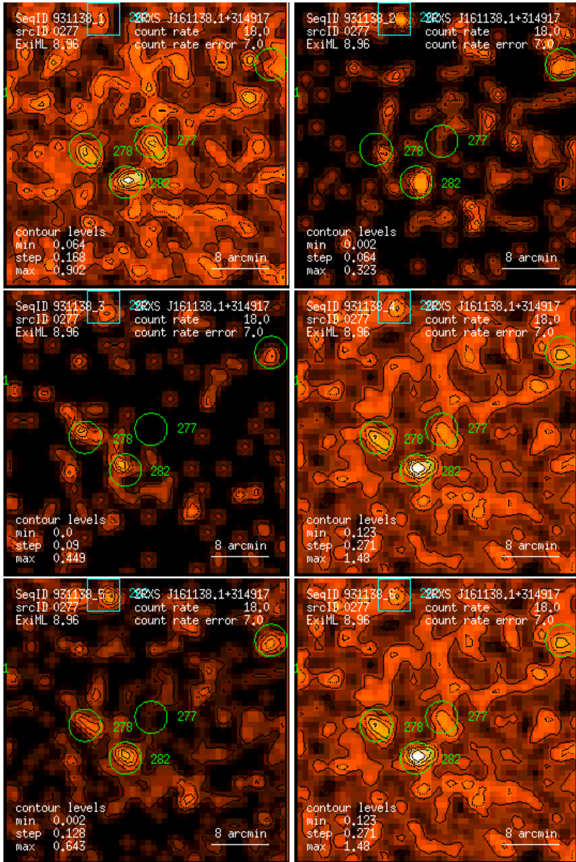
Figure 277: RASS 931138: detection 0277: band rate images, Gaussian filter: (1) PSPC channels 11 – 41, (2) 52 – 90, (3) 91 – 201, (4) 11 – 235, (5) 52 – 201, (6) 11 – 201. Broad band rates in counts/ks. Band rate contour levels in counts/ks/arcmin 2 .
