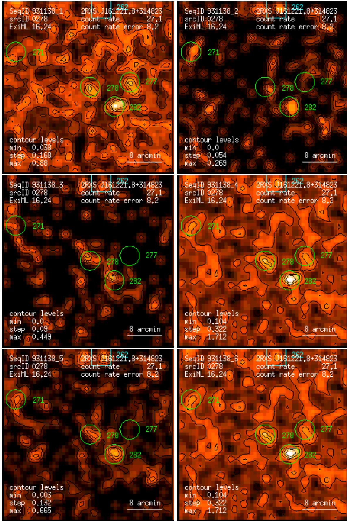
Figure 278: RASS 931138: detection 0278: band rate images, Gaussian filter: (1) PSPC channels 11 – 41, (2) 52 – 90, (3) 91 – 201, (4) 11 – 235, (5) 52 – 201, (6) 11 – 201. Broad band rates in counts/ks. Band rate contour levels in counts/ks/arcmin 2 .
