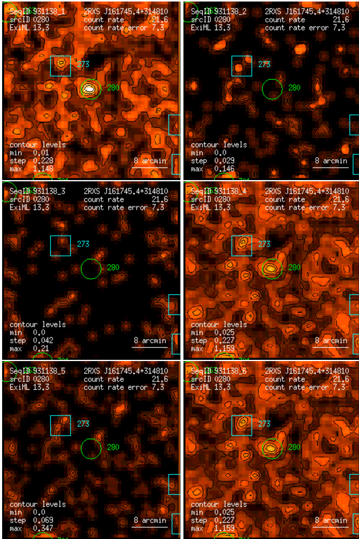
Figure 280: RASS 931138: detection 0280: band rate images, Gaussian filter: (1) PSPC channels 11 – 41, (2) 52 – 90, (3) 91 – 201, (4) 11 – 235, (5) 52 – 201, (6) 11 – 201. Broad band rates in counts/ks. Band rate contour levels in counts/ks/arcmin 2 .
