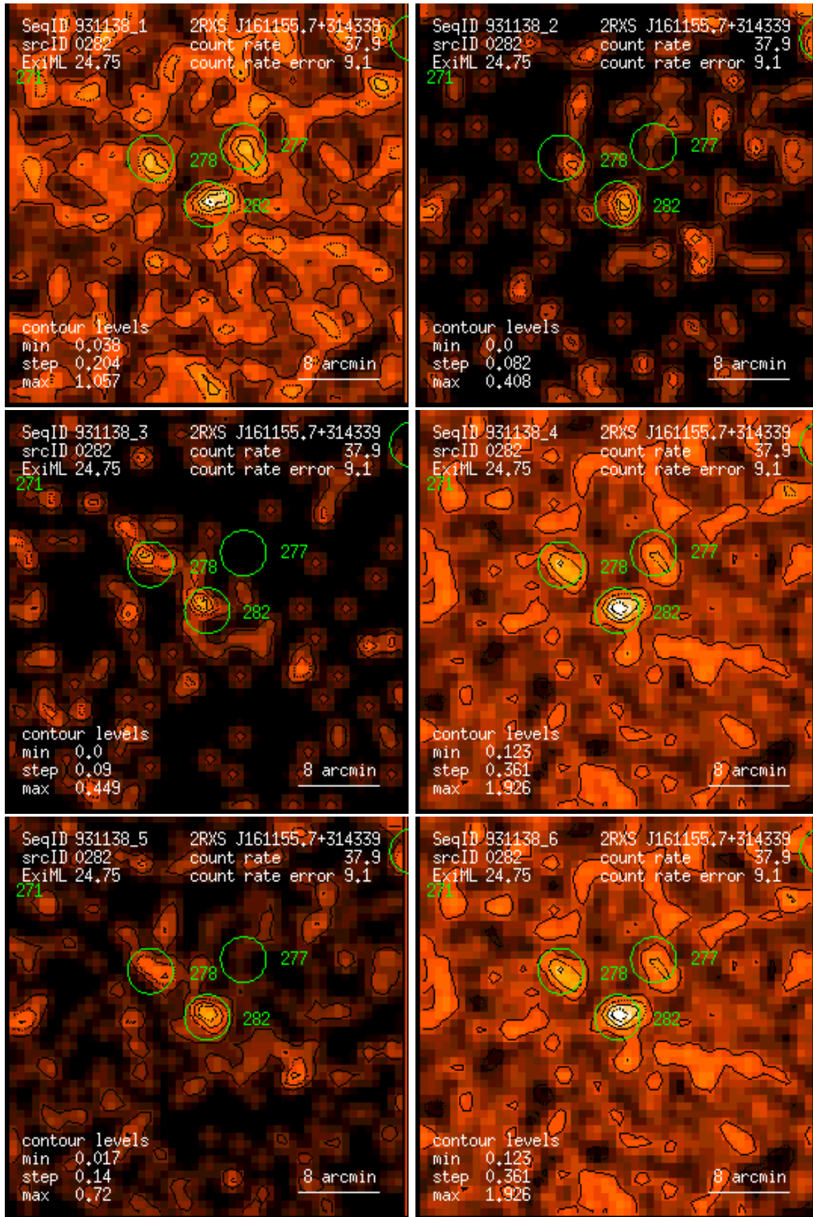
Figure 282: RASS 931138: detection 0282: band rate images, Gaussian filter: (1) PSPC channels 11 – 41, (2) 52 – 90, (3) 91 – 201, (4) 11 – 235, (5) 52 – 201, (6) 11 – 201. Broad band rates in counts/ks. Band rate contour levels in counts/ks/arcmin 2 .
