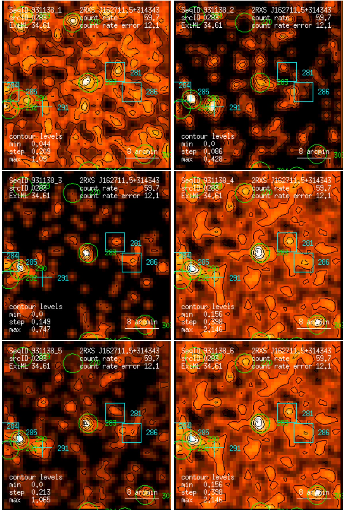
Figure 283: RASS 931138: detection 0283: band rate images, Gaussian filter: (1) PSPC channels 11 – 41, (2) 52 – 90, (3) 91 – 201, (4) 11 – 235, (5) 52 – 201, (6) 11 – 201. Broad band rates in counts/ks. Band rate contour levels in counts/ks/arcmin 2 .
