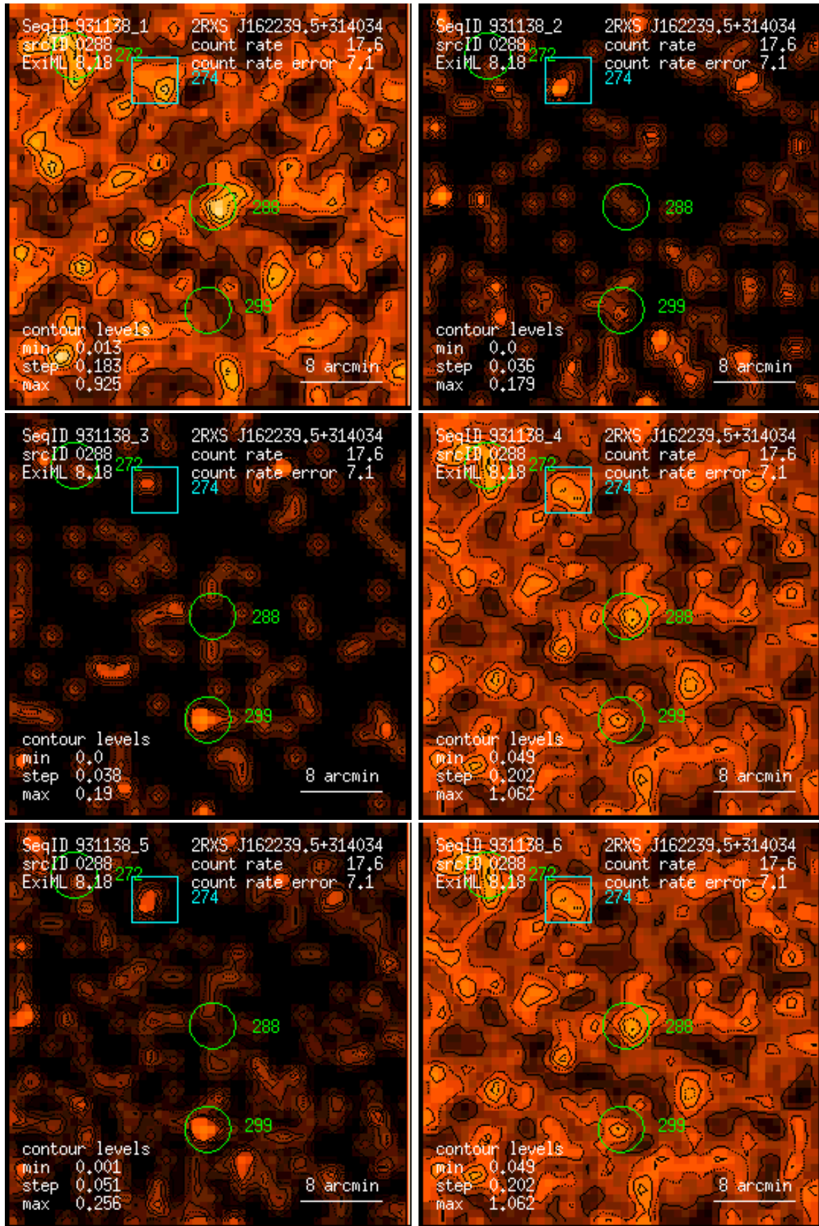
Figure 288: RASS 931138: detection 0288: band rate images, Gaussian filter: (1) PSPC channels 11 – 41, (2) 52 – 90, (3) 91 – 201, (4) 11 – 235, (5) 52 – 201, (6) 11 – 201. Broad band rates in counts/ks. Band rate contour levels in counts/ks/arcmin 2 .
