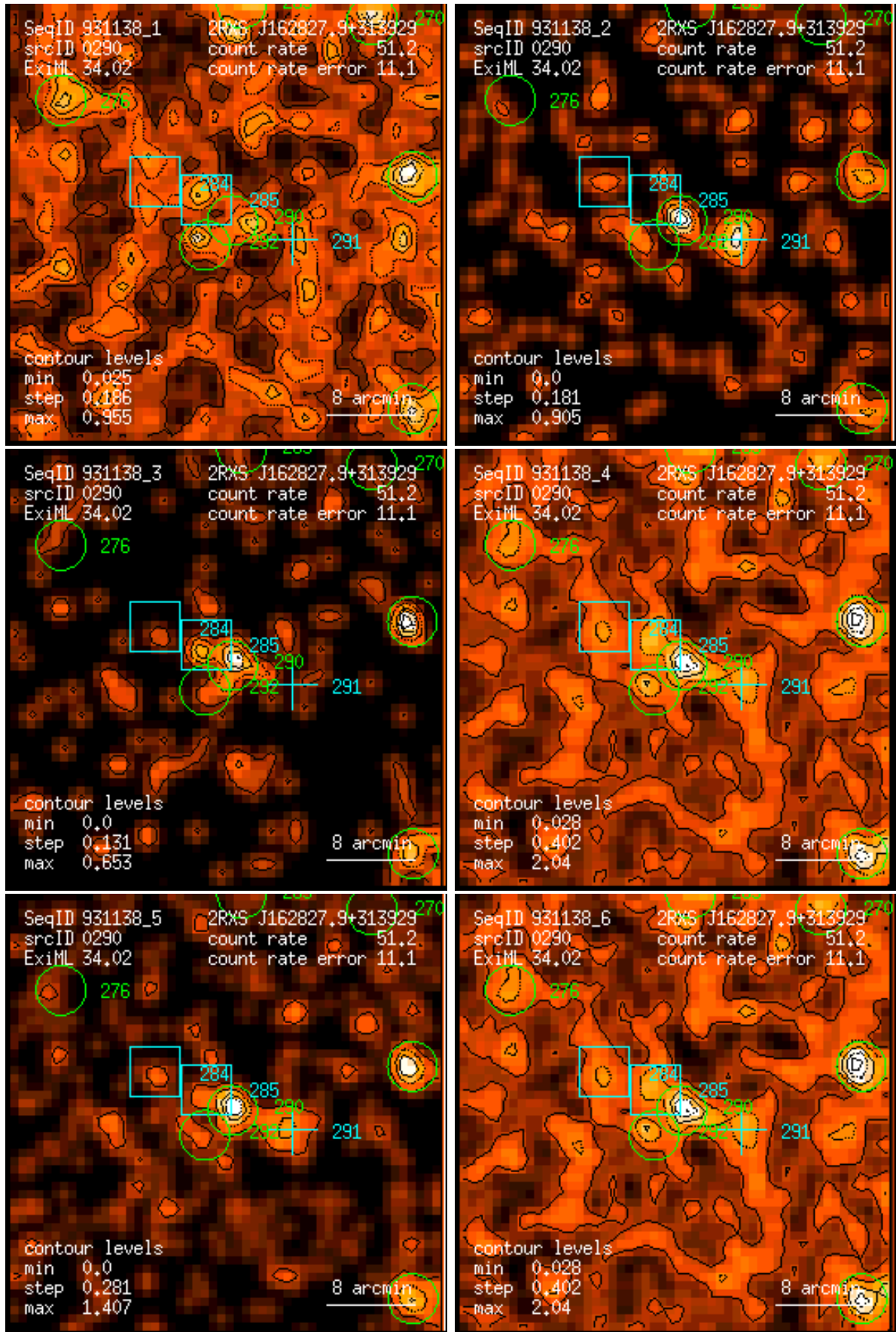
Figure 290: RASS 931138: detection 0290: band rate images, Gaussian filter: (1) PSPC channels 11 – 41, (2) 52 – 90, (3) 91 – 201, (4) 11 – 235, (5) 52 – 201, (6) 11 – 201. Broad band rates in counts/ks. Band rate contour levels in counts/ks/arcmin 2 .
