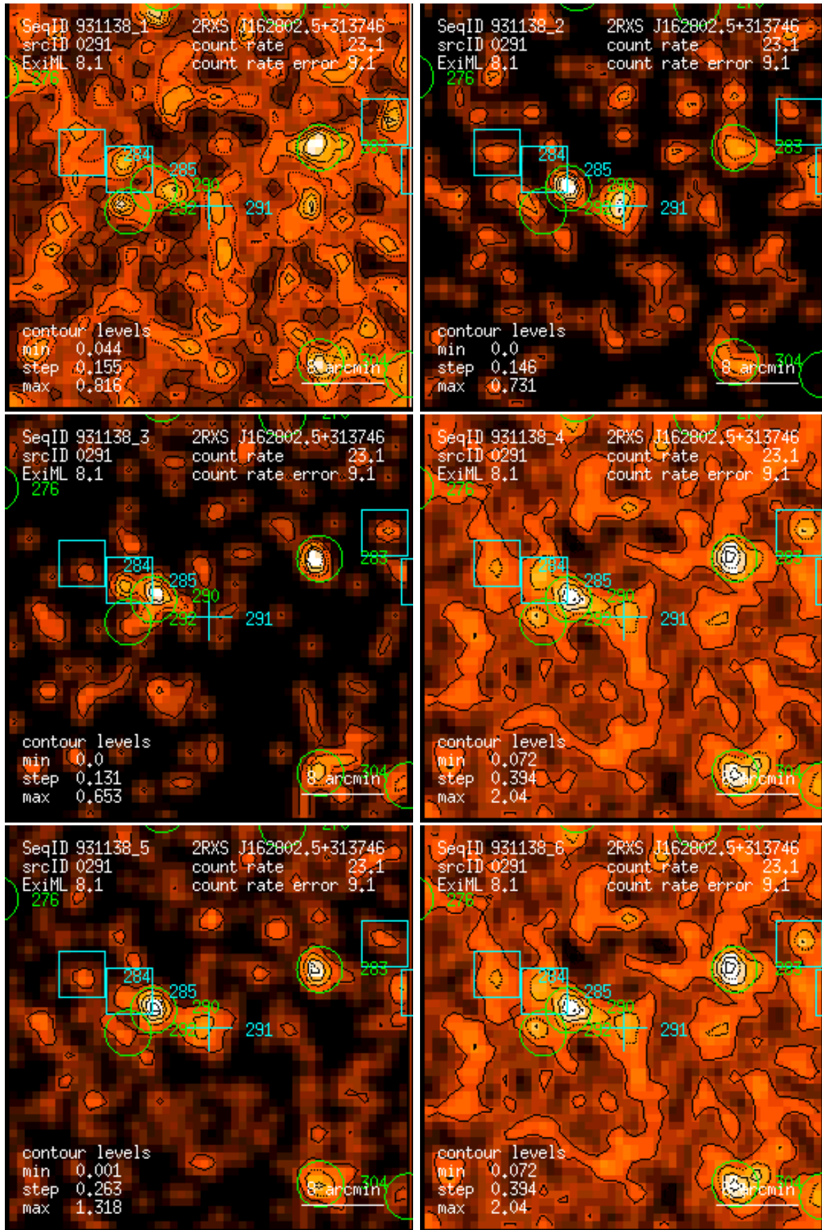
Figure 291: RASS 931138: detection 0291: band rate images, Gaussian filter: (1) PSPC channels 11 – 41, (2) 52 – 90, (3) 91 – 201, (4) 11 – 235, (5) 52 – 201, (6) 11 – 201. Broad band rates in counts/ks. Band rate contour levels in counts/ks/arcmin 2 .
