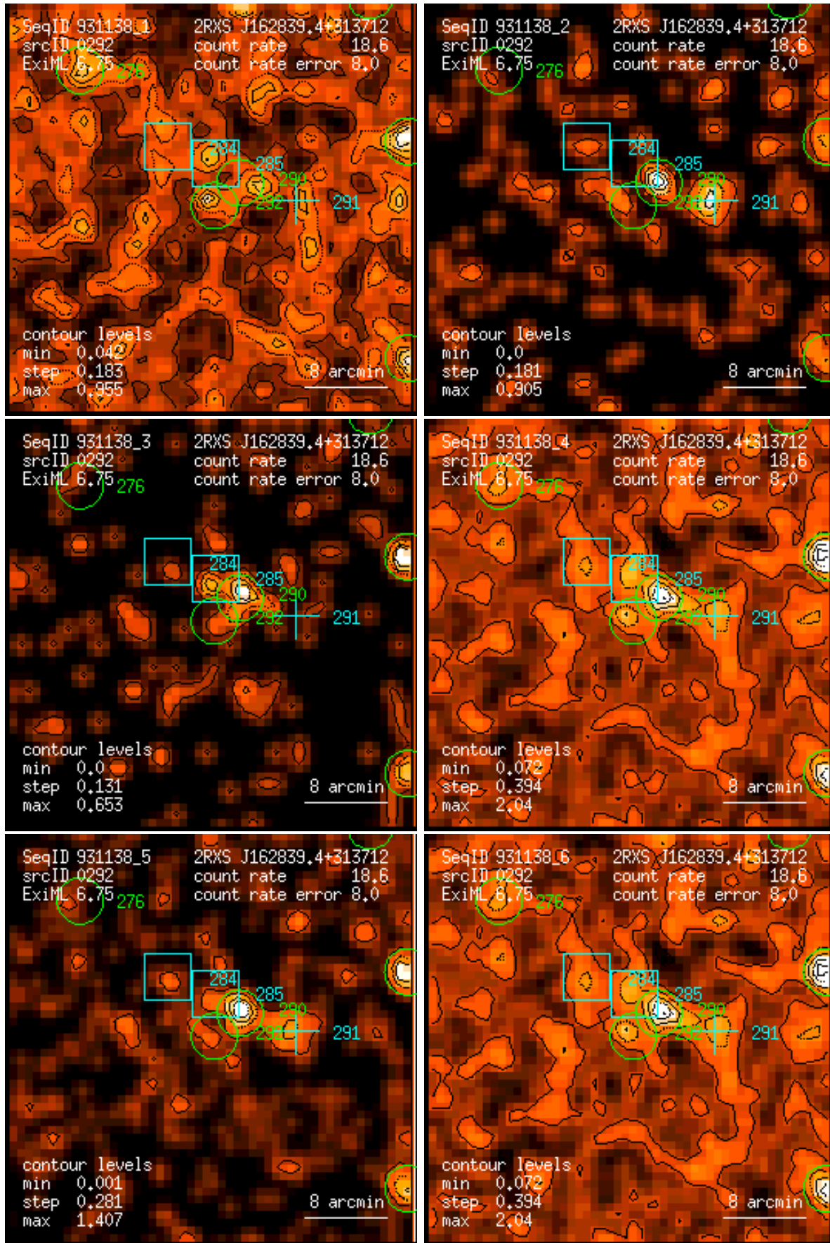
Figure 292: RASS 931138: detection 0292: band rate images, Gaussian filter: (1) PSPC channels 11 – 41, (2) 52 – 90, (3) 91 – 201, (4) 11 – 235, (5) 52 – 201, (6) 11 – 201. Broad band rates in counts/ks. Band rate contour levels in counts/ks/arcmin 2 .
