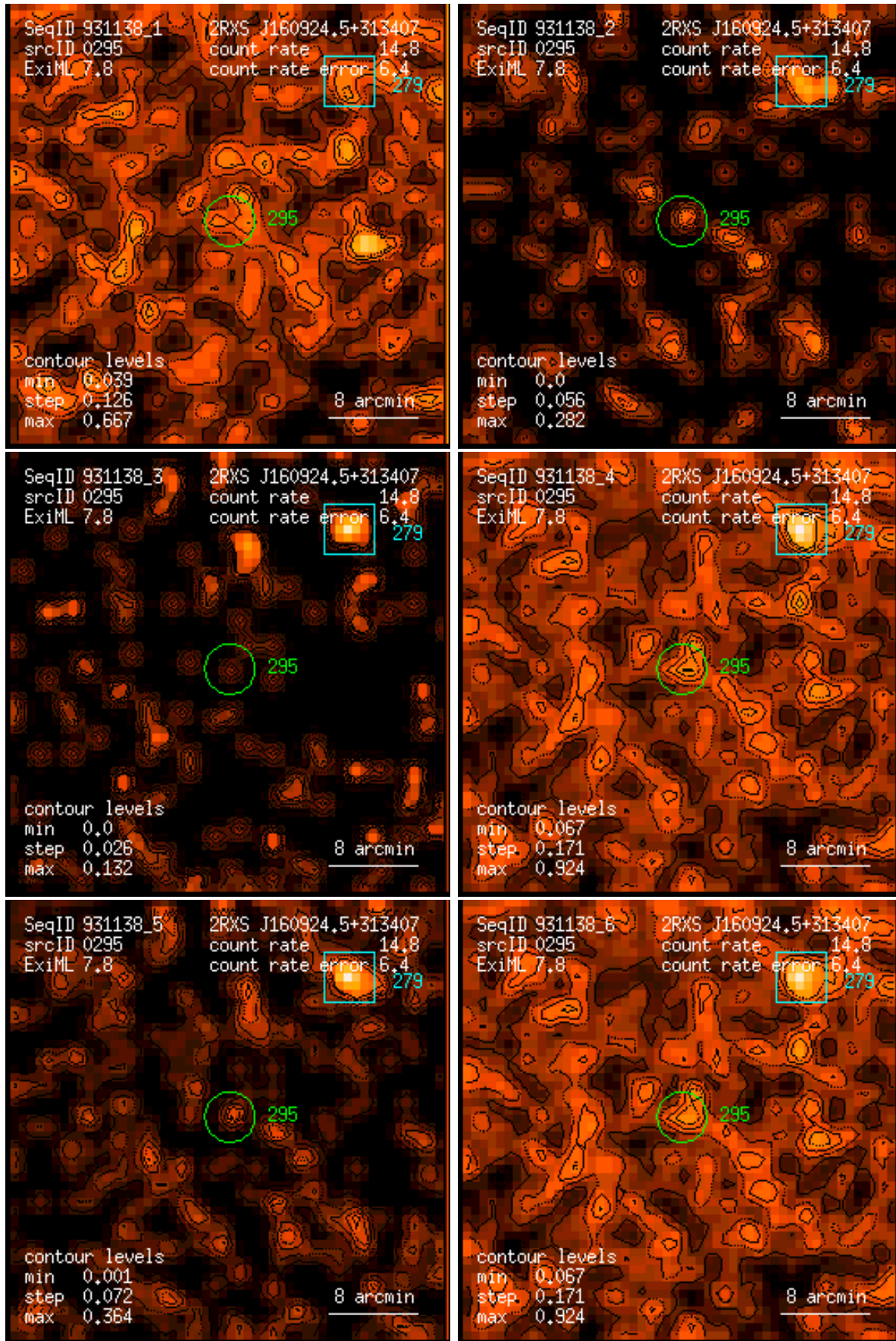
Figure 295: RASS 931138: detection 0295: band rate images, Gaussian filter: (1) PSPC channels 11 – 41, (2) 52 – 90, (3) 91 – 201, (4) 11 – 235, (5) 52 – 201, (6) 11 – 201. Broad band rates in counts/ks. Band rate contour levels in counts/ks/arcmin 2 .
