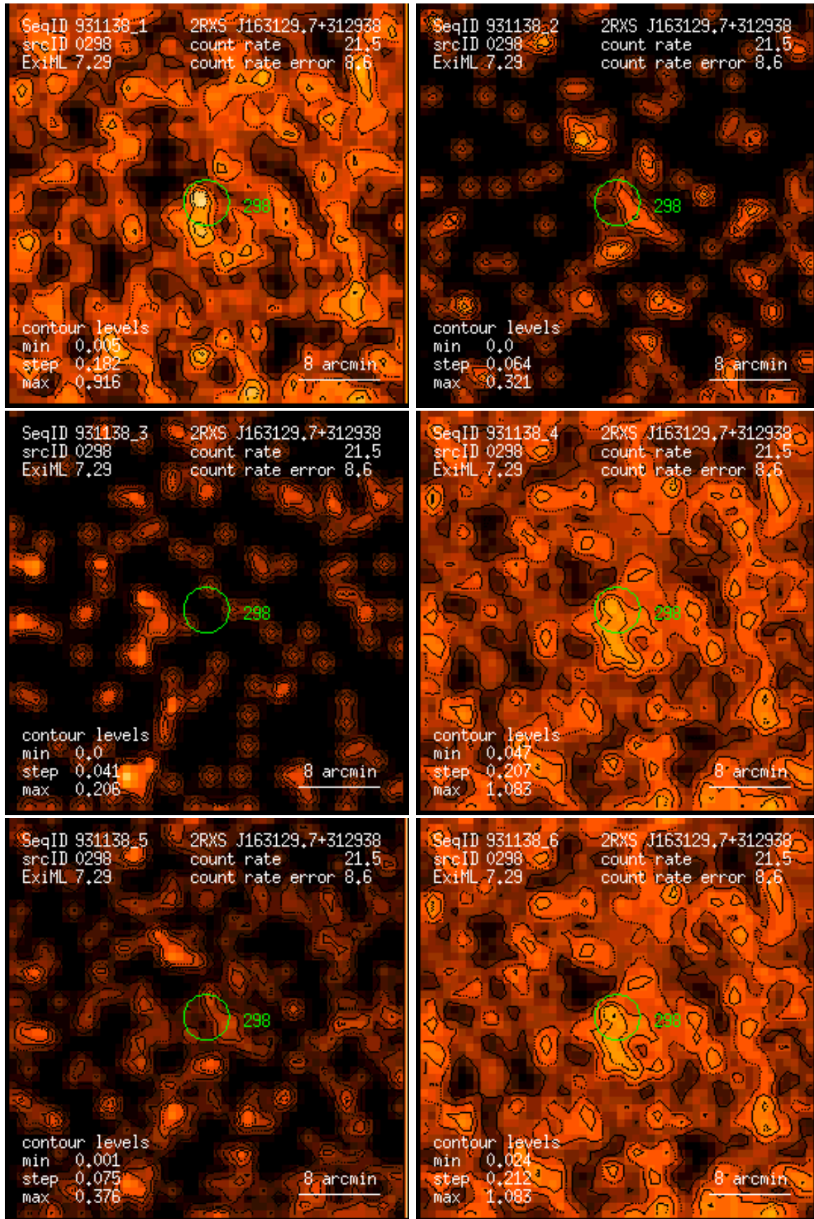
Figure 298: RASS 931138: detection 0298: band rate images, Gaussian filter: (1) PSPC channels 11 – 41, (2) 52 – 90, (3) 91 – 201, (4) 11 – 235, (5) 52 – 201, (6) 11 – 201. Broad band rates in counts/ks. Band rate contour levels in counts/ks/arcmin 2 .
