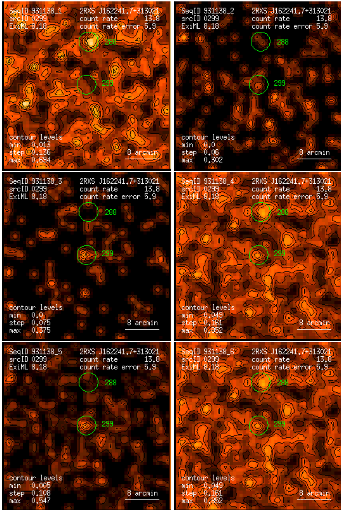
Figure 299: RASS 931138: detection 0299: band rate images, Gaussian filter: (1) PSPC channels 11 – 41, (2) 52 – 90, (3) 91 – 201, (4) 11 – 235, (5) 52 – 201, (6) 11 – 201. Broad band rates in counts/ks. Band rate contour levels in counts/ks/arcmin 2 .
