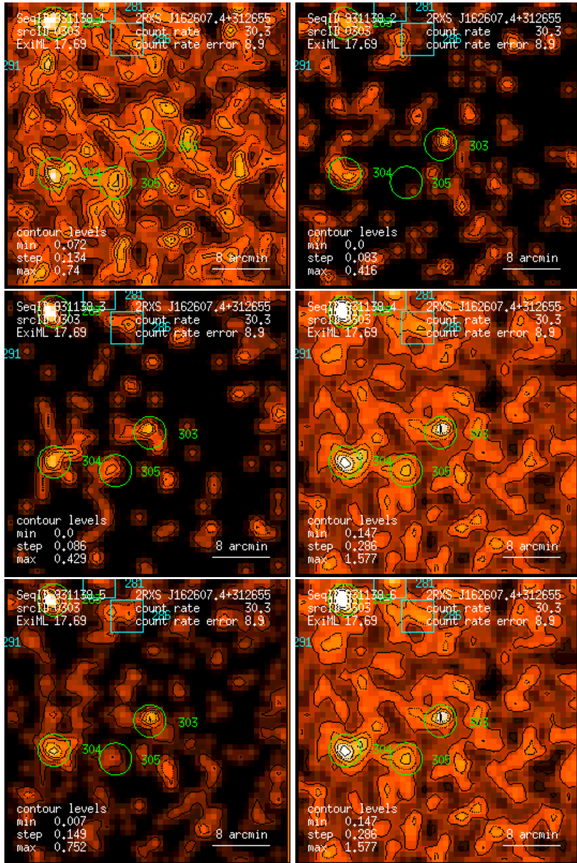
Figure 303: RASS 931138: detection 0303: band rate images, Gaussian filter: (1) PSPC channels 11 – 41, (2) 52 – 90, (3) 91 – 201, (4) 11 – 235, (5) 52 – 201, (6) 11 – 201. Broad band rates in counts/ks. Band rate contour levels in counts/ks/arcmin 2 .
