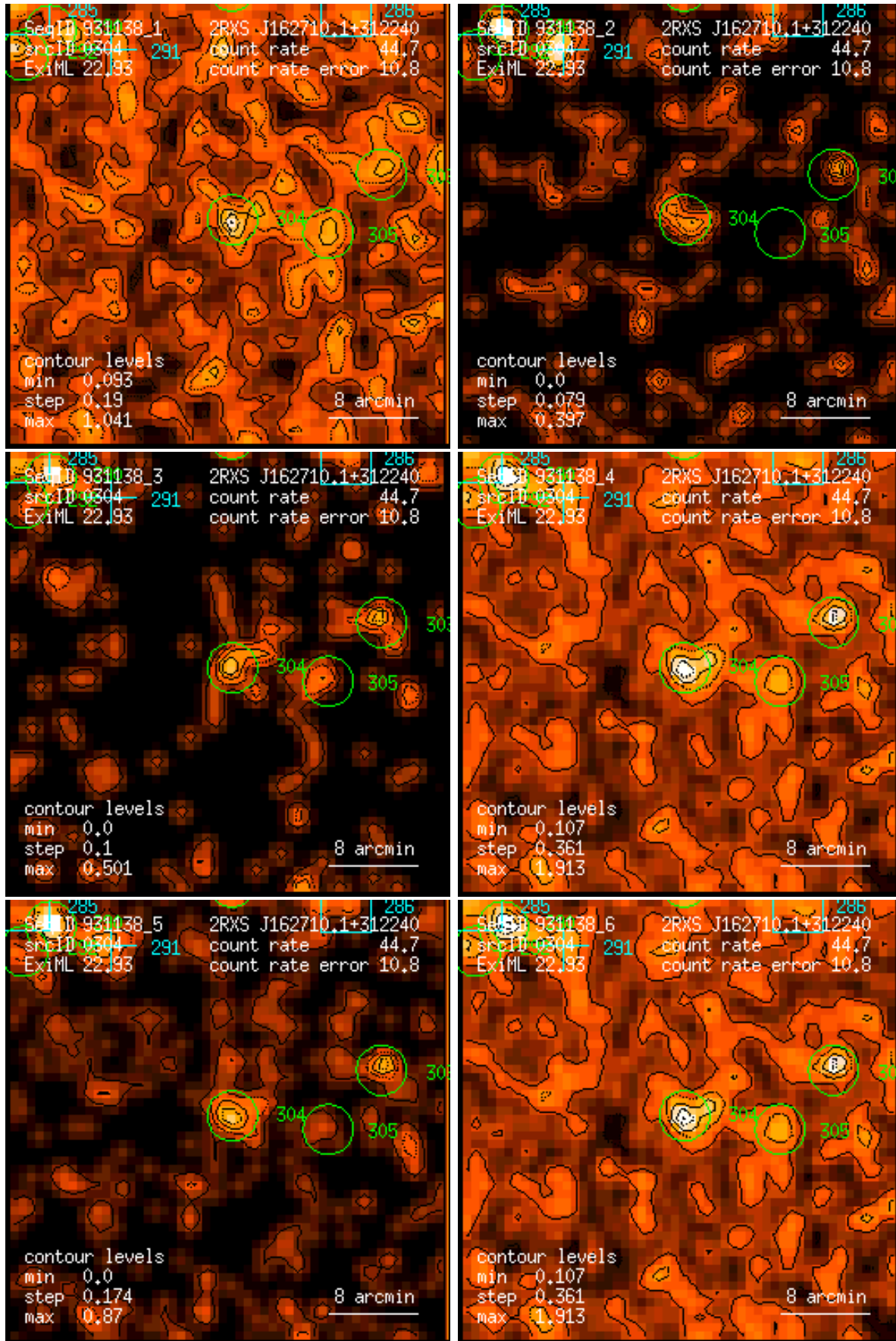
Figure 304: RASS 931138: detection 0304: band rate images, Gaussian filter: (1) PSPC channels 11 – 41, (2) 52 – 90, (3) 91 – 201, (4) 11 – 235, (5) 52 – 201, (6) 11 – 201. Broad band rates in counts/ks. Band rate contour levels in counts/ks/arcmin 2 .
