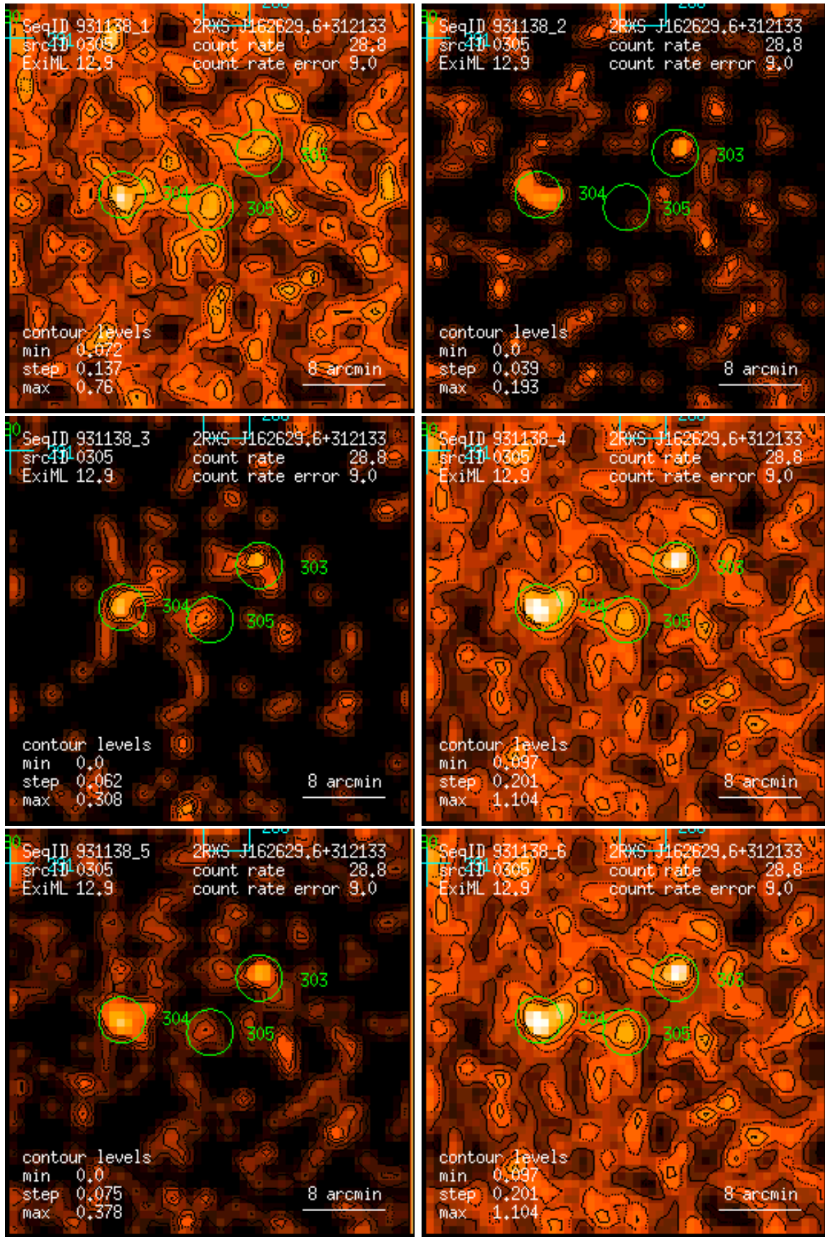
Figure 305: RASS 931138: detection 0305: band rate images, Gaussian filter: (1) PSPC channels 11 – 41, (2) 52 – 90, (3) 91 – 201, (4) 11 – 235, (5) 52 – 201, (6) 11 – 201. Broad band rates in counts/ks. Band rate contour levels in counts/ks/arcmin 2 .
