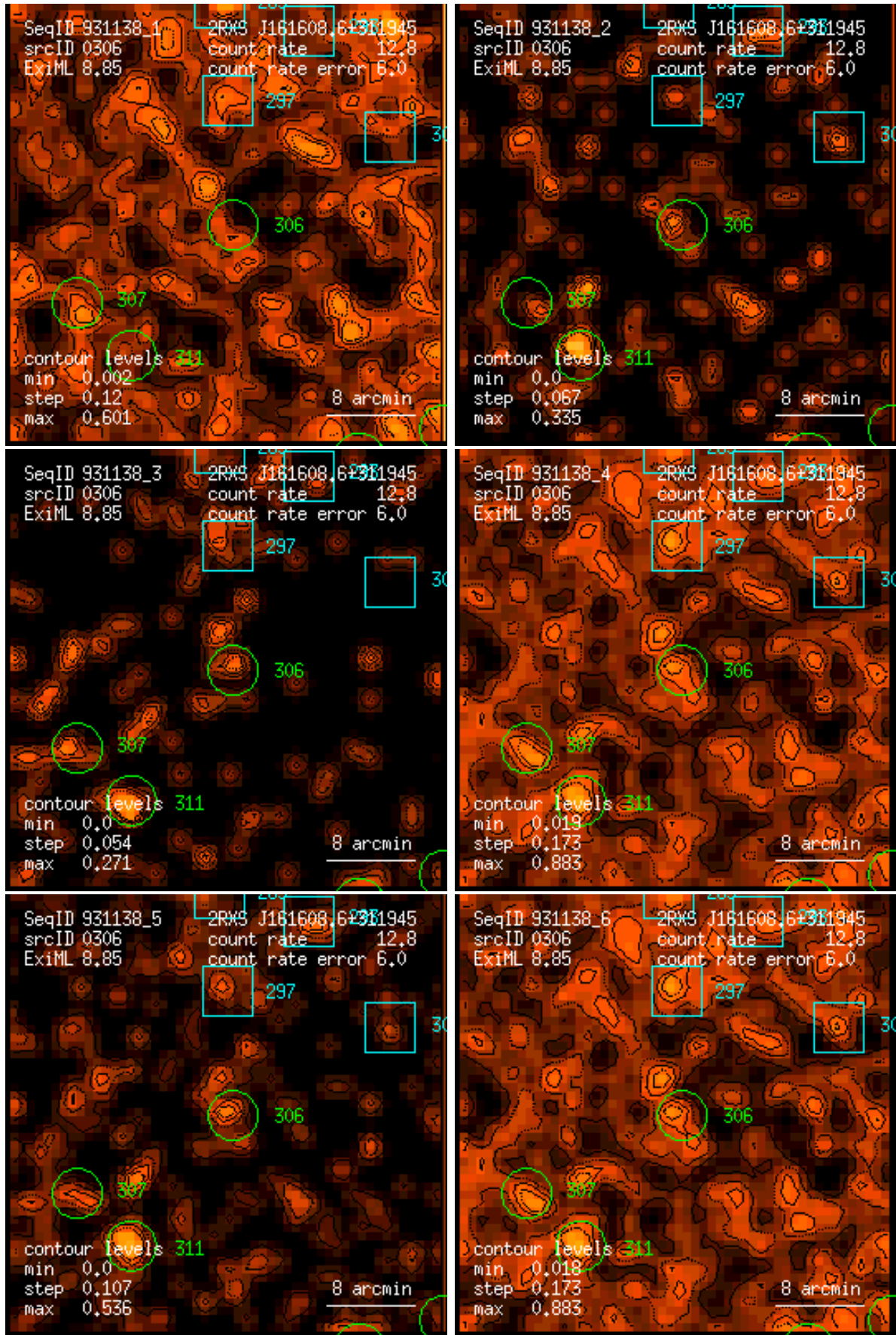
Figure 306: RASS 931138: detection 0306: band rate images, Gaussian filter: (1) PSPC channels 11 – 41, (2) 52 – 90, (3) 91 – 201, (4) 11 – 235, (5) 52 – 201, (6) 11 – 201. Broad band rates in counts/ks. Band rate contour levels in counts/ks/arcmin 2 .
