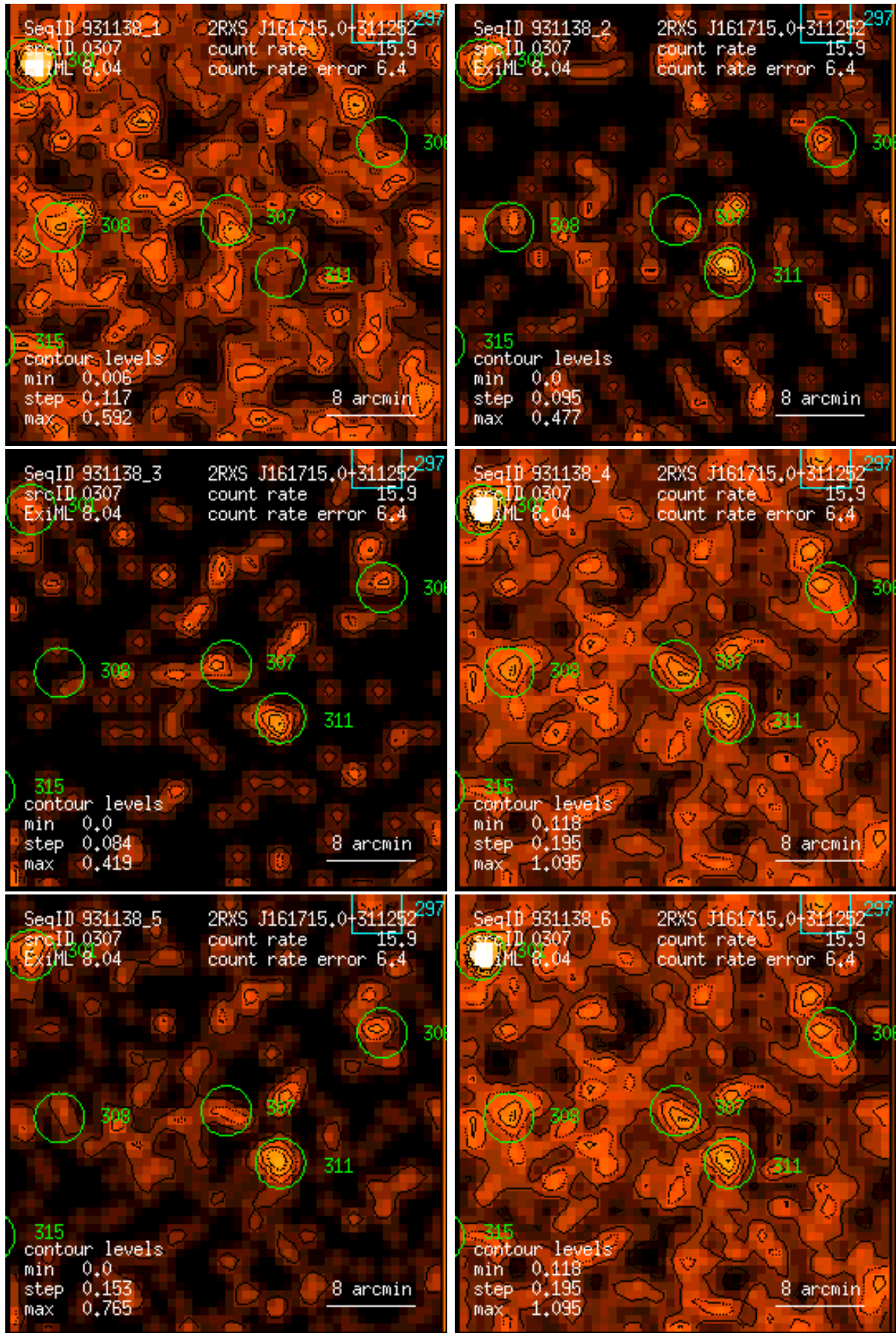
Figure 307: RASS 931138: detection 0307: band rate images, Gaussian filter: (1) PSPC channels 11 – 41, (2) 52 – 90, (3) 91 – 201, (4) 11 – 235, (5) 52 – 201, (6) 11 – 201. Broad band rates in counts/ks. Band rate contour levels in counts/ks/arcmin 2 .
