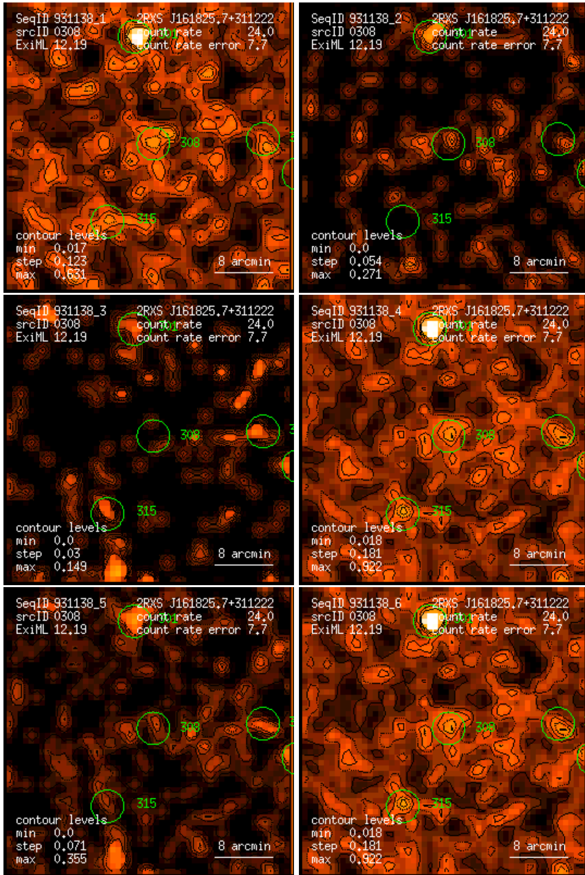
Figure 308: RASS 931138: detection 0308: band rate images, Gaussian filter: (1) PSPC channels 11 – 41, (2) 52 – 90, (3) 91 – 201, (4) 11 – 235, (5) 52 – 201, (6) 11 – 201. Broad band rates in counts/ks. Band rate contour levels in counts/ks/arcmin 2 .
