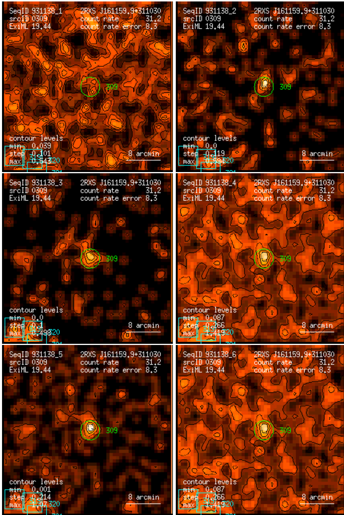
Figure 309: RASS 931138: detection 0309: band rate images, Gaussian filter: (1) PSPC channels 11 – 41, (2) 52 – 90, (3) 91 – 201, (4) 11 – 235, (5) 52 – 201, (6) 11 – 201. Broad band rates in counts/ks. Band rate contour levels in counts/ks/arcmin 2 .
