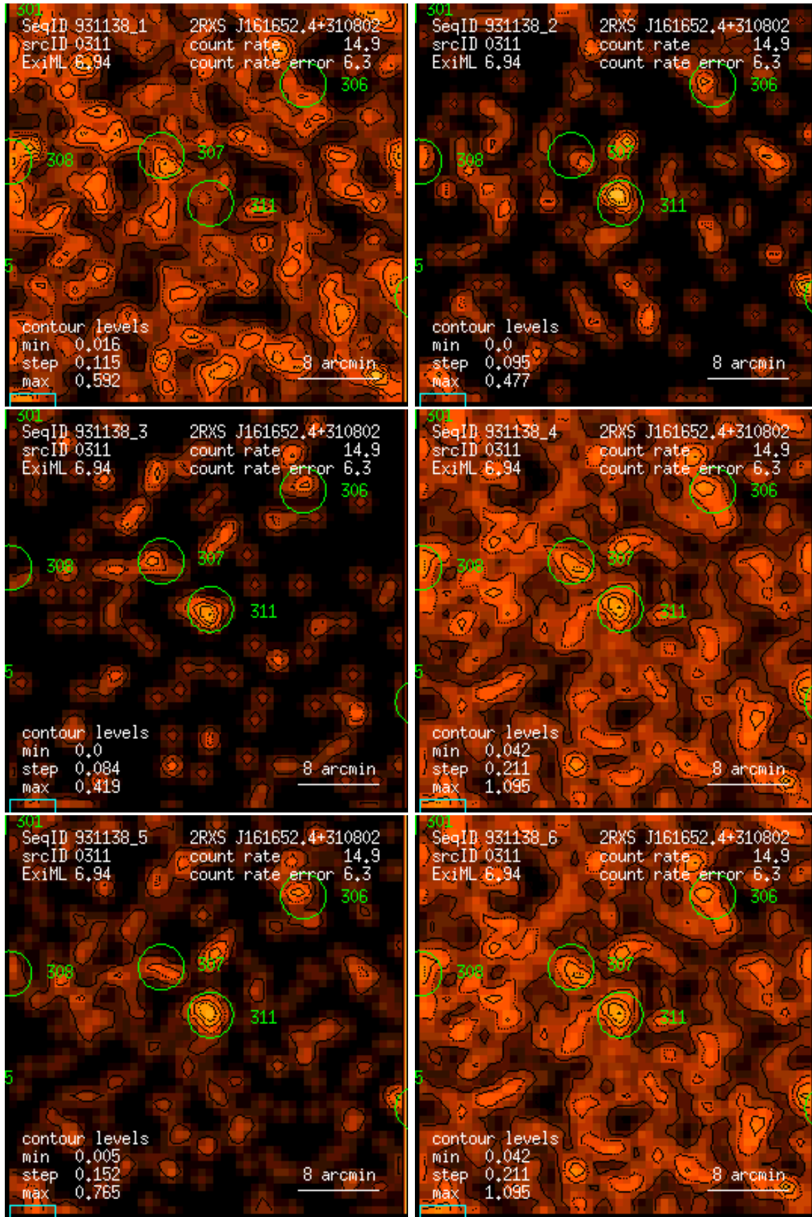
Figure 311: RASS 931138: detection 0311: band rate images, Gaussian filter: (1) PSPC channels 11 – 41, (2) 52 – 90, (3) 91 – 201, (4) 11 – 235, (5) 52 – 201, (6) 11 – 201. Broad band rates in counts/ks. Band rate contour levels in counts/ks/arcmin 2 .
