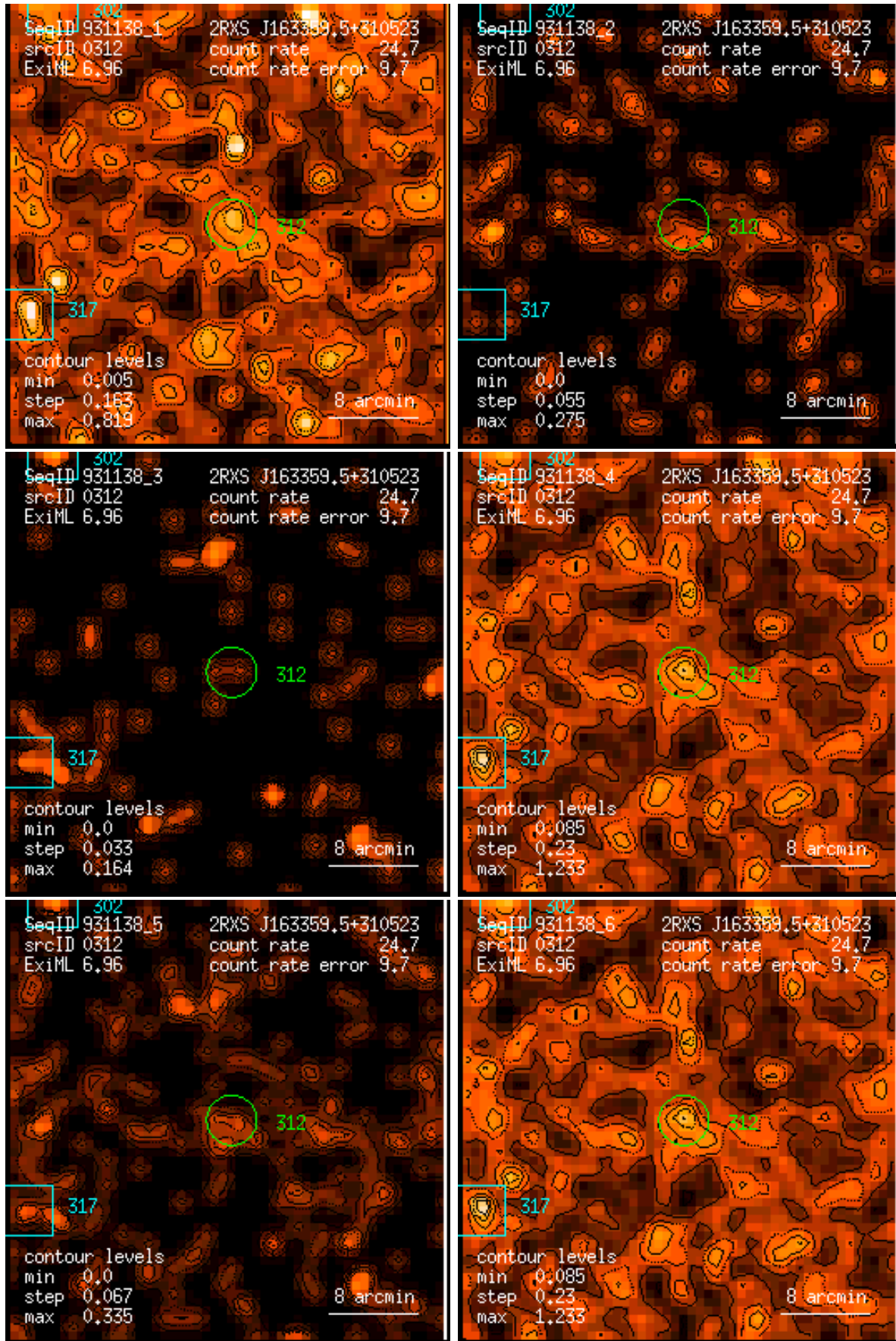
Figure 312: RASS 931138: detection 0312: band rate images, Gaussian filter: (1) PSPC channels 11 – 41, (2) 52 – 90, (3) 91 – 201, (4) 11 – 235, (5) 52 – 201, (6) 11 – 201. Broad band rates in counts/ks. Band rate contour levels in counts/ks/arcmin 2 .
