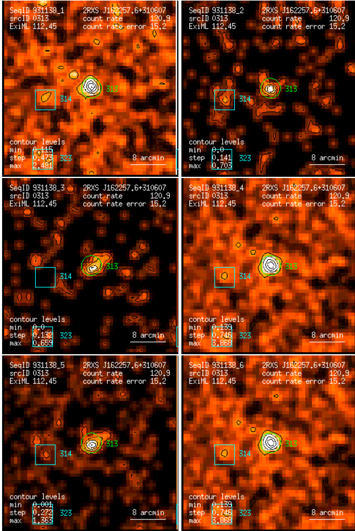
Figure 313: RASS 931138: detection 0313: band rate images, Gaussian filter: (1) PSPC channels 11 – 41, (2) 52 – 90, (3) 91 – 201, (4) 11 – 235, (5) 52 – 201, (6) 11 – 201. Broad band rates in counts/ks. Band rate contour levels in counts/ks/arcmin 2 .
