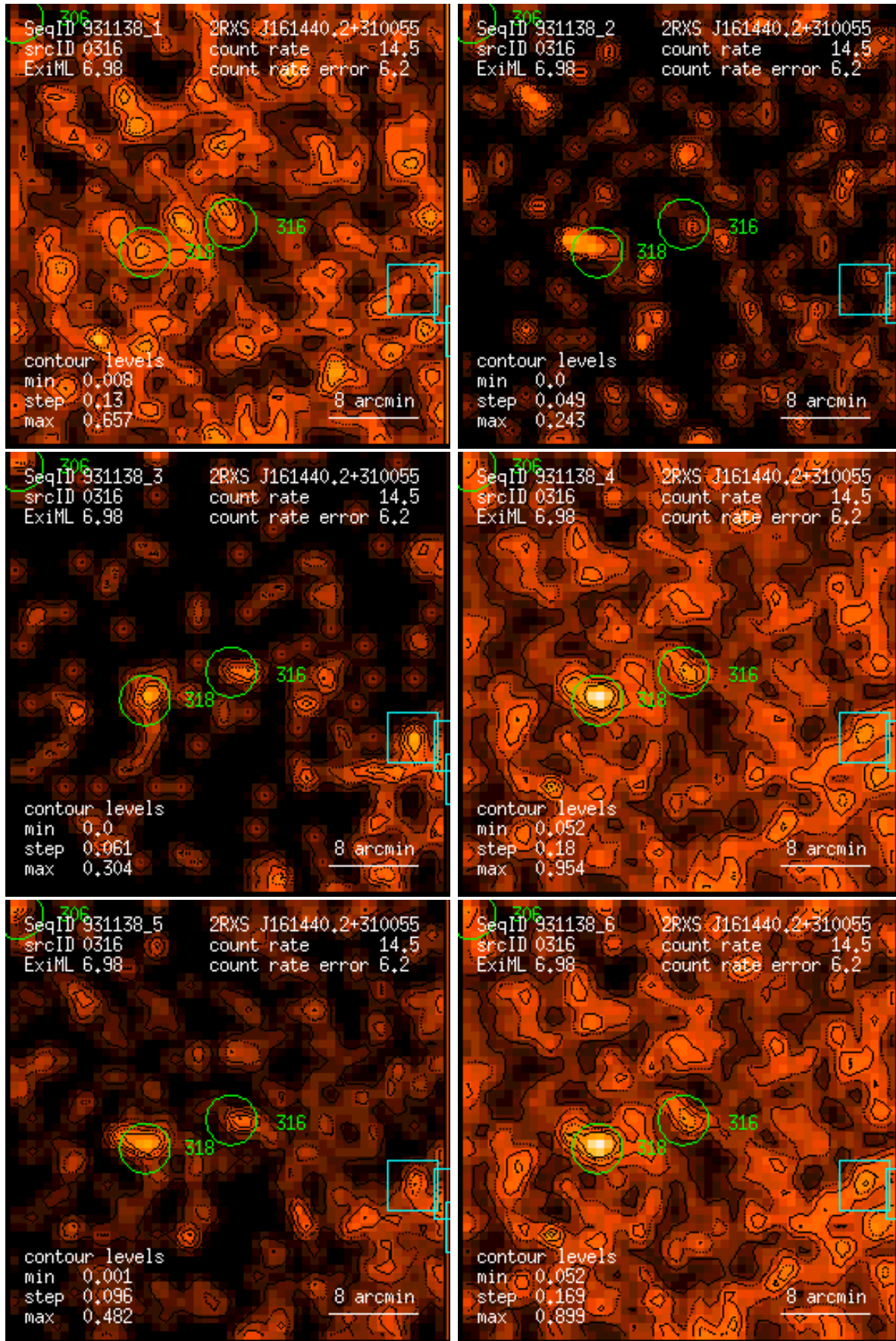
Figure 316: RASS 931138: detection 0316: band rate images, Gaussian filter: (1) PSPC channels 11 – 41, (2) 52 – 90, (3) 91 – 201, (4) 11 – 235, (5) 52 – 201, (6) 11 – 201. Broad band rates in counts/ks. Band rate contour levels in counts/ks/arcmin 2 .
