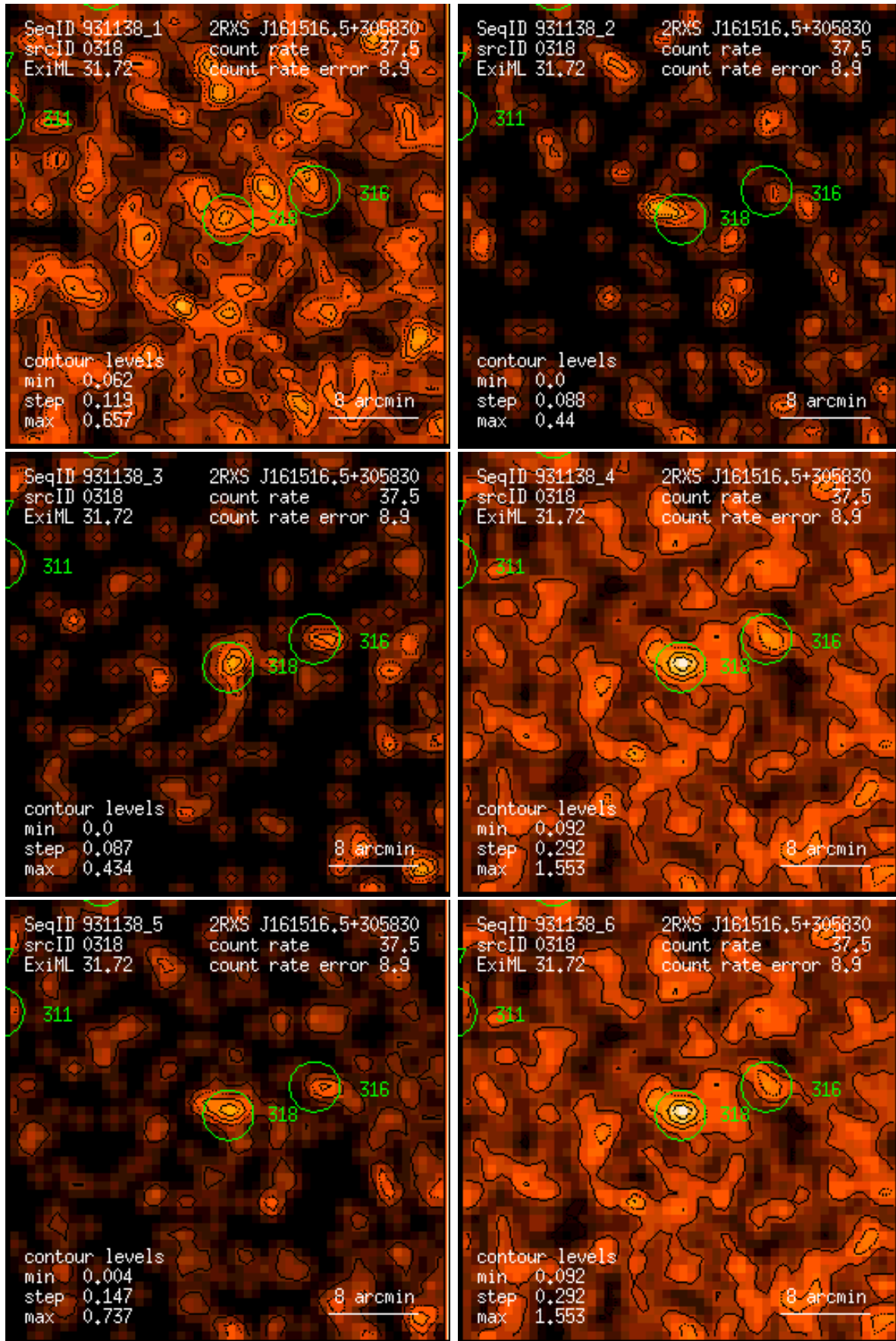
Figure 318: RASS 931138: detection 0318: band rate images, Gaussian filter: (1) PSPC channels 11 – 41, (2) 52 – 90, (3) 91 – 201, (4) 11 – 235, (5) 52 – 201, (6) 11 – 201. Broad band rates in counts/ks. Band rate contour levels in counts/ks/arcmin 2 .
