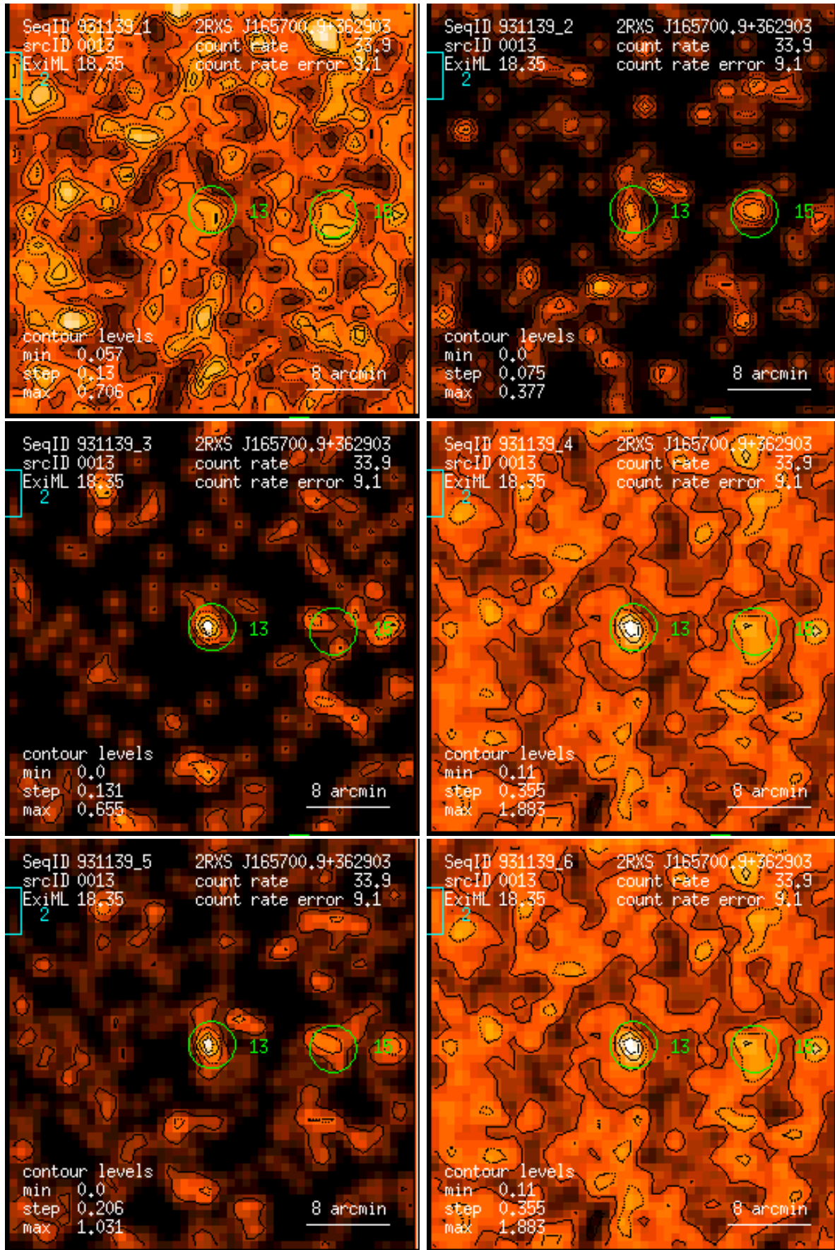
Figure 13: RASS 931139: detection 0013: band rate images, Gaussian filter: (1) PSPC channels 11 – 41, (2) 52 – 90, (3) 91 – 201, (4) 11 – 235, (5) 52 – 201, (6) 11 – 201. Broad band rates in counts/ks. Band rate contour levels in counts/ks/arcmin 2 .
