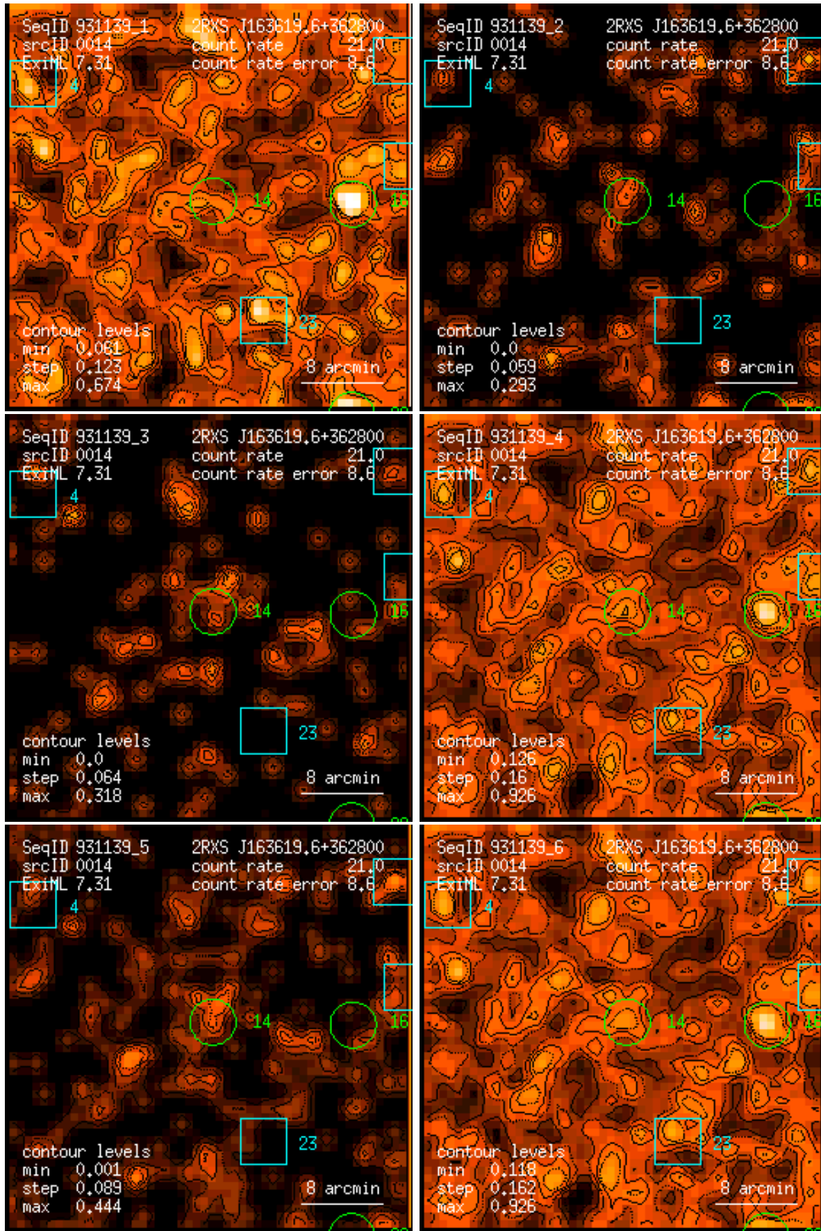
Figure 14: RASS 931139: detection 0014: band rate images, Gaussian filter: (1) PSPC channels 11 – 41, (2) 52 – 90, (3) 91 – 201, (4) 11 – 235, (5) 52 – 201, (6) 11 – 201. Broad band rates in counts/ks. Band rate contour levels in counts/ks/arcmin 2 .
