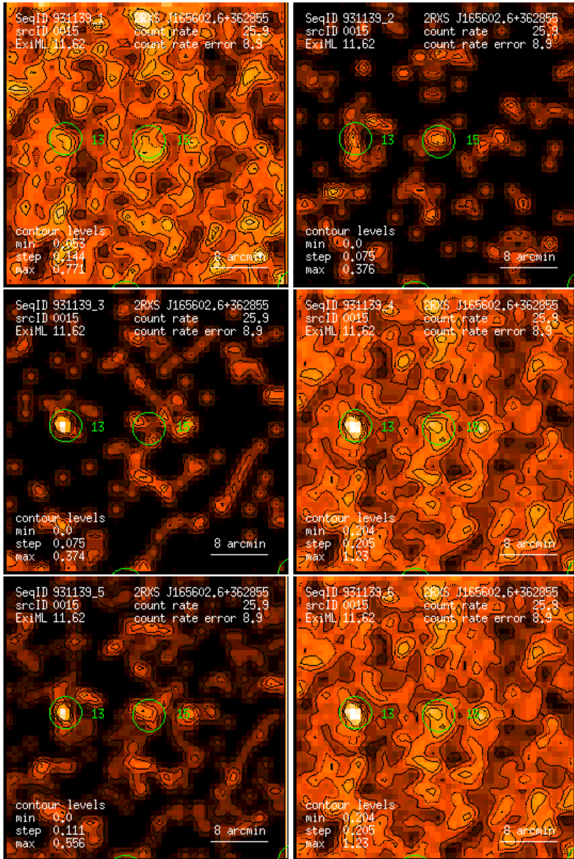
Figure 15: RASS 931139: detection 0015: band rate images, Gaussian filter: (1) PSPC channels 11 – 41, (2) 52 – 90, (3) 91 – 201, (4) 11 – 235, (5) 52 – 201, (6) 11 – 201. Broad band rates in counts/ks. Band rate contour levels in counts/ks/arcmin 2 .
