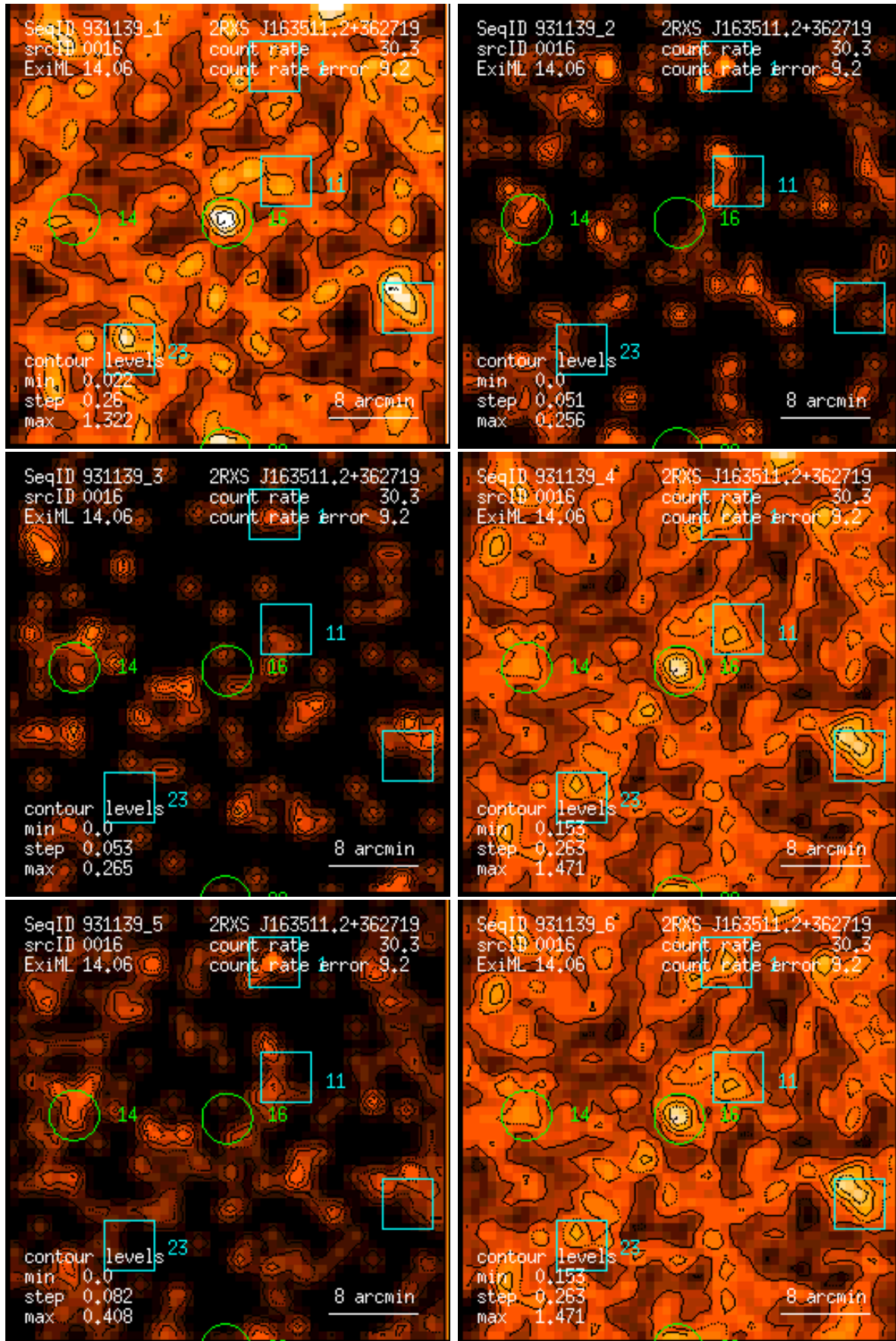
Figure 16: RASS 931139: detection 0016: band rate images, Gaussian filter: (1) PSPC channels 11 – 41, (2) 52 – 90, (3) 91 – 201, (4) 11 – 235, (5) 52 – 201, (6) 11 – 201. Broad band rates in counts/ks. Band rate contour levels in counts/ks/arcmin 2 .
