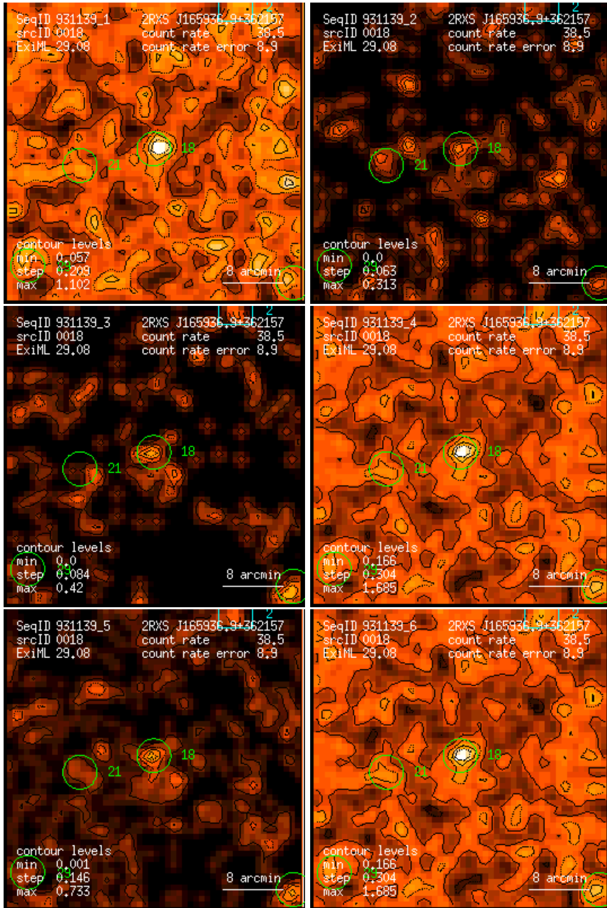
Figure 18: RASS 931139: detection 0018: band rate images, Gaussian filter: (1) PSPC channels 11 – 41, (2) 52 – 90, (3) 91 – 201, (4) 11 – 235, (5) 52 – 201, (6) 11 – 201. Broad band rates in counts/ks. Band rate contour levels in counts/ks/arcmin 2 .
