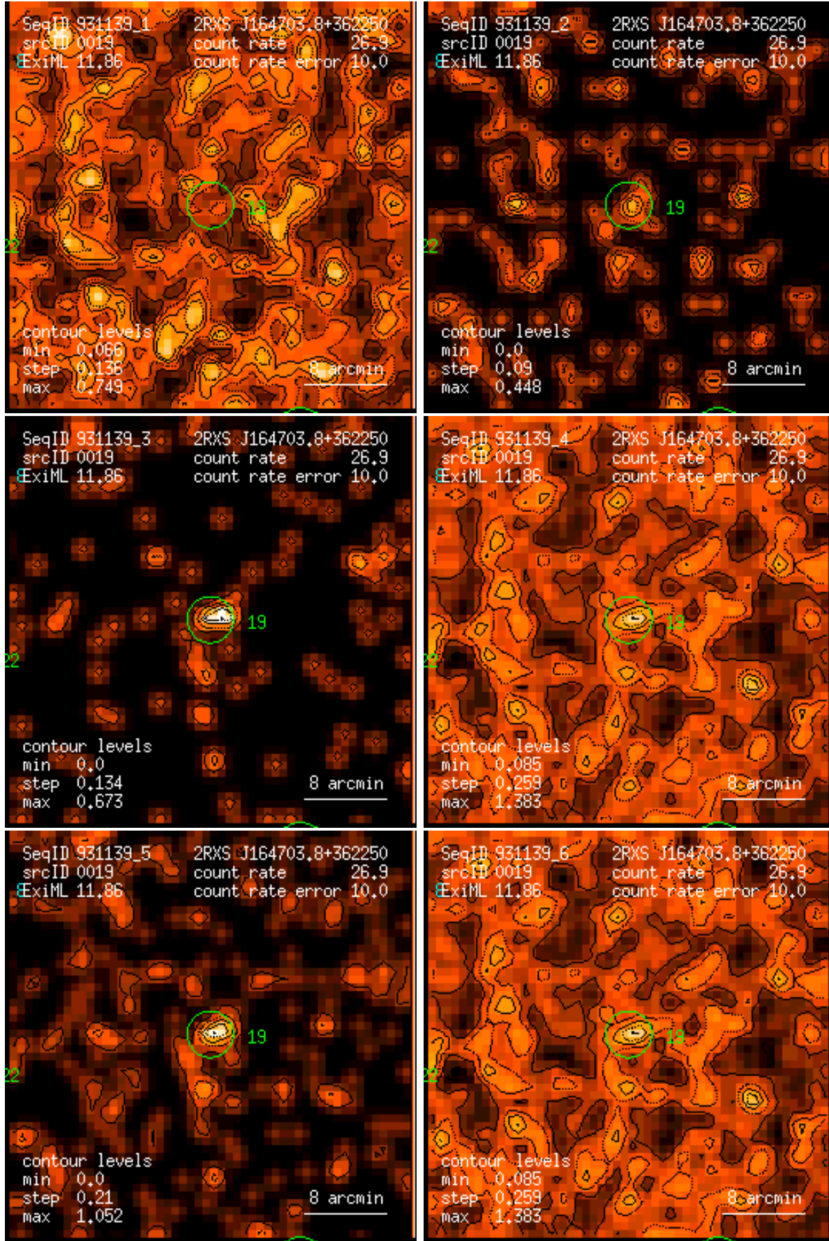
Figure 19: RASS 931139: detection 0019: band rate images, Gaussian filter: (1) PSPC channels 11 – 41, (2) 52 – 90, (3) 91 – 201, (4) 11 – 235, (5) 52 – 201, (6) 11 – 201. Broad band rates in counts/ks. Band rate contour levels in counts/ks/arcmin 2 .
