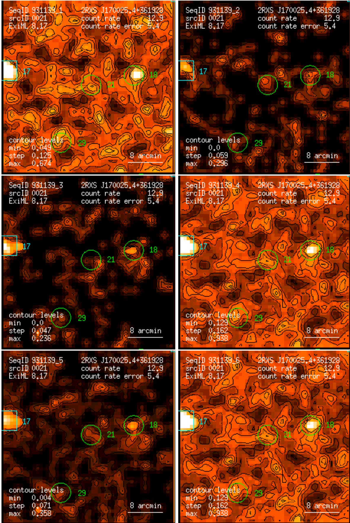
Figure 21: RASS 931139: detection 0021: band rate images, Gaussian filter: (1) PSPC channels 11 – 41, (2) 52 – 90, (3) 91 – 201, (4) 11 – 235, (5) 52 – 201, (6) 11 – 201. Broad band rates in counts/ks. Band rate contour levels in counts/ks/arcmin 2 .
