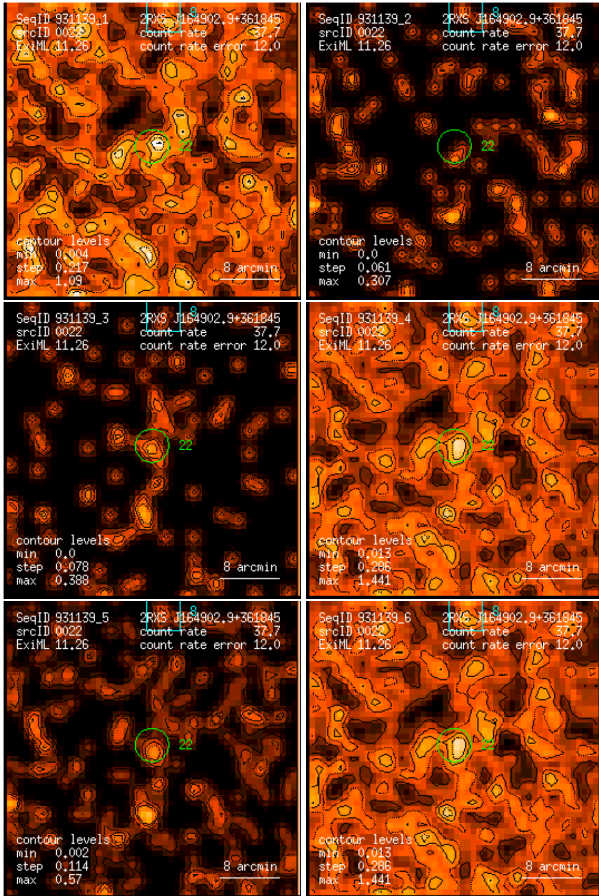
Figure 22: RASS 931139: detection 0022: band rate images, Gaussian filter: (1) PSPC channels 11 – 41, (2) 52 – 90, (3) 91 – 201, (4) 11 – 235, (5) 52 – 201, (6) 11 – 201. Broad band rates in counts/ks. Band rate contour levels in counts/ks/arcmin 2 .
