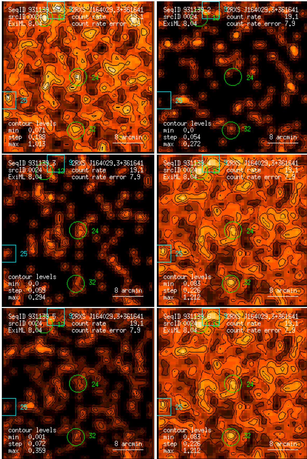
Figure 24: RASS 931139: detection 0024: band rate images, Gaussian filter: (1) PSPC channels 11 – 41, (2) 52 – 90, (3) 91 – 201, (4) 11 – 235, (5) 52 – 201, (6) 11 – 201. Broad band rates in counts/ks. Band rate contour levels in counts/ks/arcmin 2 .
