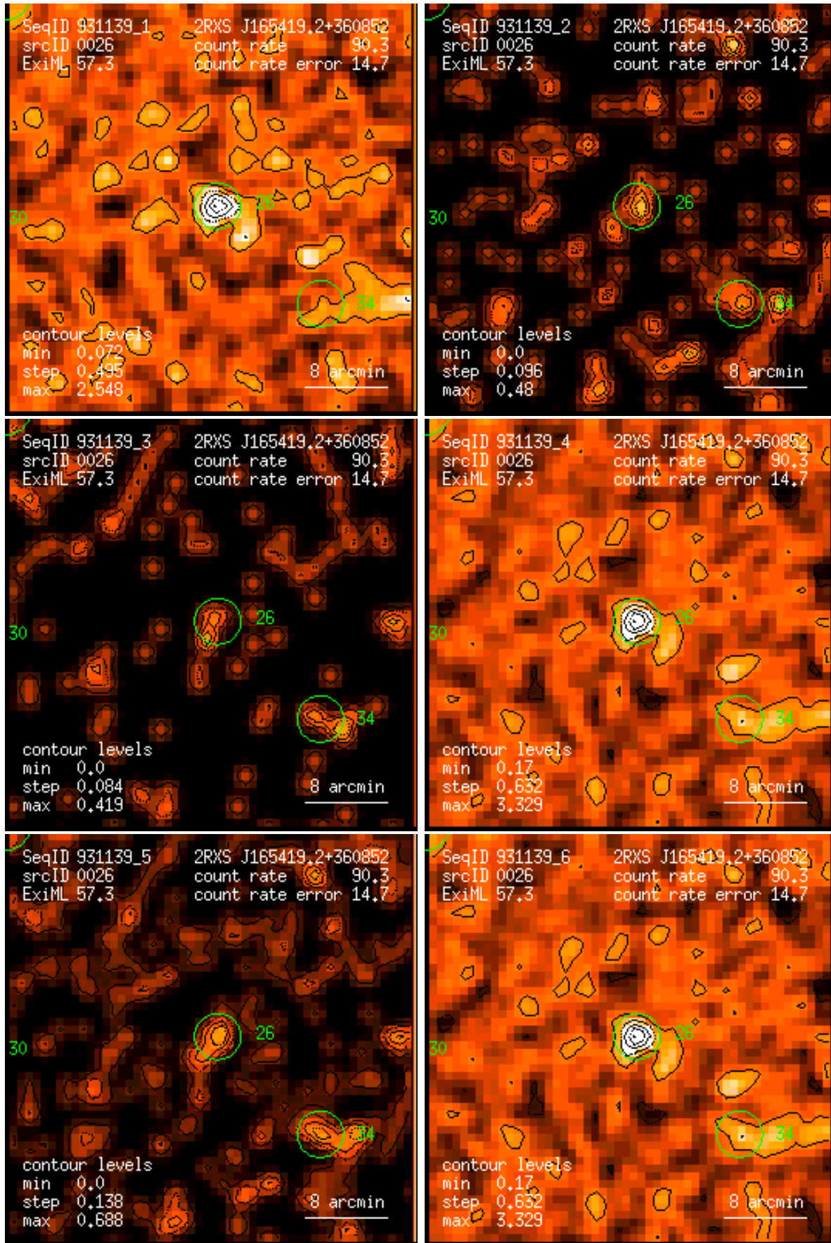
Figure 26: RASS 931139: detection 0026: band rate images, Gaussian filter: (1) PSPC channels 11 – 41, (2) 52 – 90, (3) 91 – 201, (4) 11 – 235, (5) 52 – 201, (6) 11 – 201. Broad band rates in counts/ks. Band rate contour levels in counts/ks/arcmin 2 .
