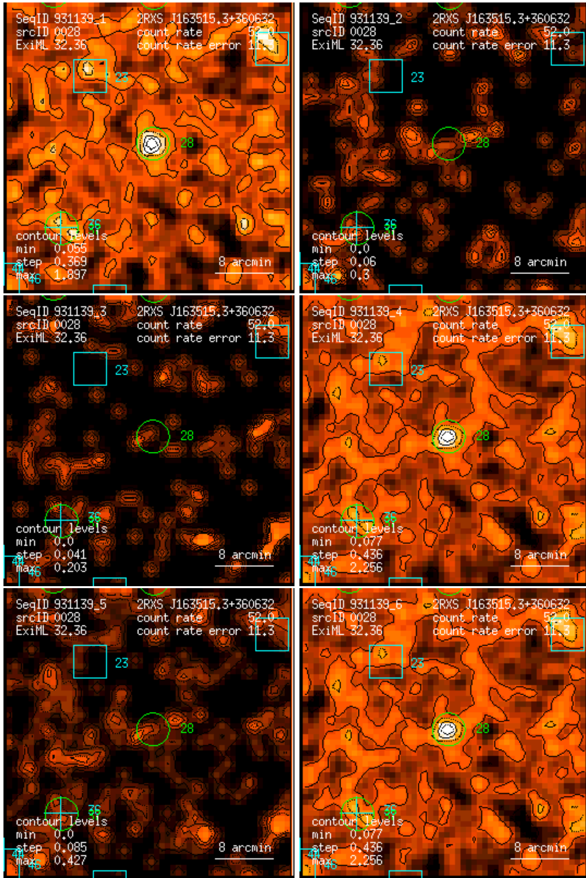
Figure 28: RASS 931139: detection 0028: band rate images, Gaussian filter: (1) PSPC channels 11 – 41, (2) 52 – 90, (3) 91 – 201, (4) 11 – 235, (5) 52 – 201, (6) 11 – 201. Broad band rates in counts/ks. Band rate contour levels in counts/ks/arcmin 2 .
