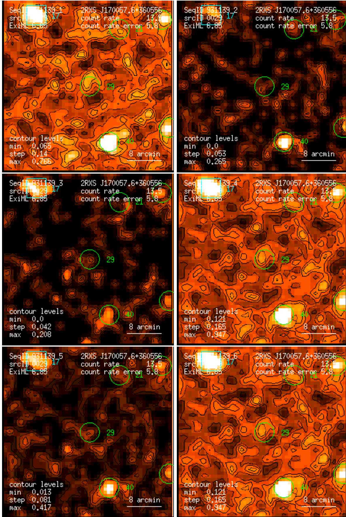
Figure 29: RASS 931139: detection 0029: band rate images, Gaussian filter: (1) PSPC channels 11 – 41, (2) 52 – 90, (3) 91 – 201, (4) 11 – 235, (5) 52 – 201, (6) 11 – 201. Broad band rates in counts/ks. Band rate contour levels in counts/ks/arcmin 2 .
