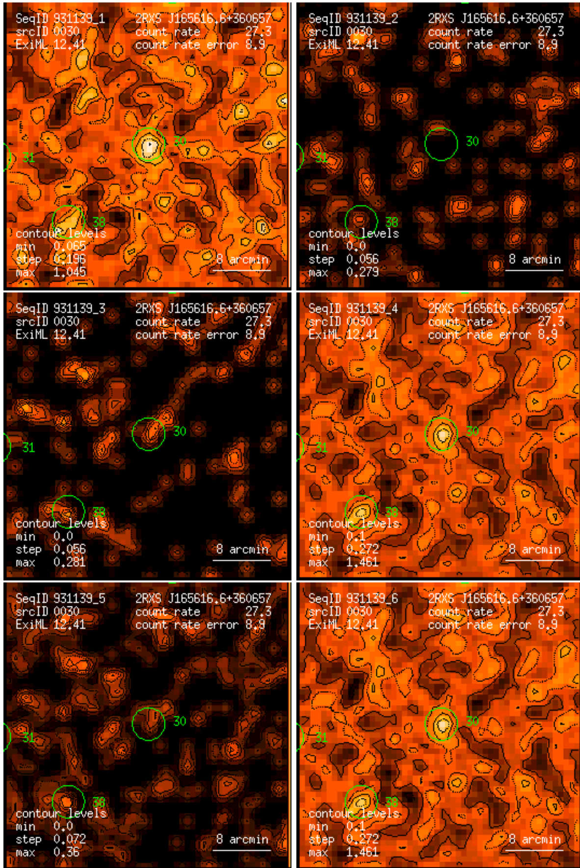
Figure 30: RASS 931139: detection 0030: band rate images, Gaussian filter: (1) PSPC channels 11 – 41, (2) 52 – 90, (3) 91 – 201, (4) 11 – 235, (5) 52 – 201, (6) 11 – 201. Broad band rates in counts/ks. Band rate contour levels in counts/ks/arcmin 2 .
