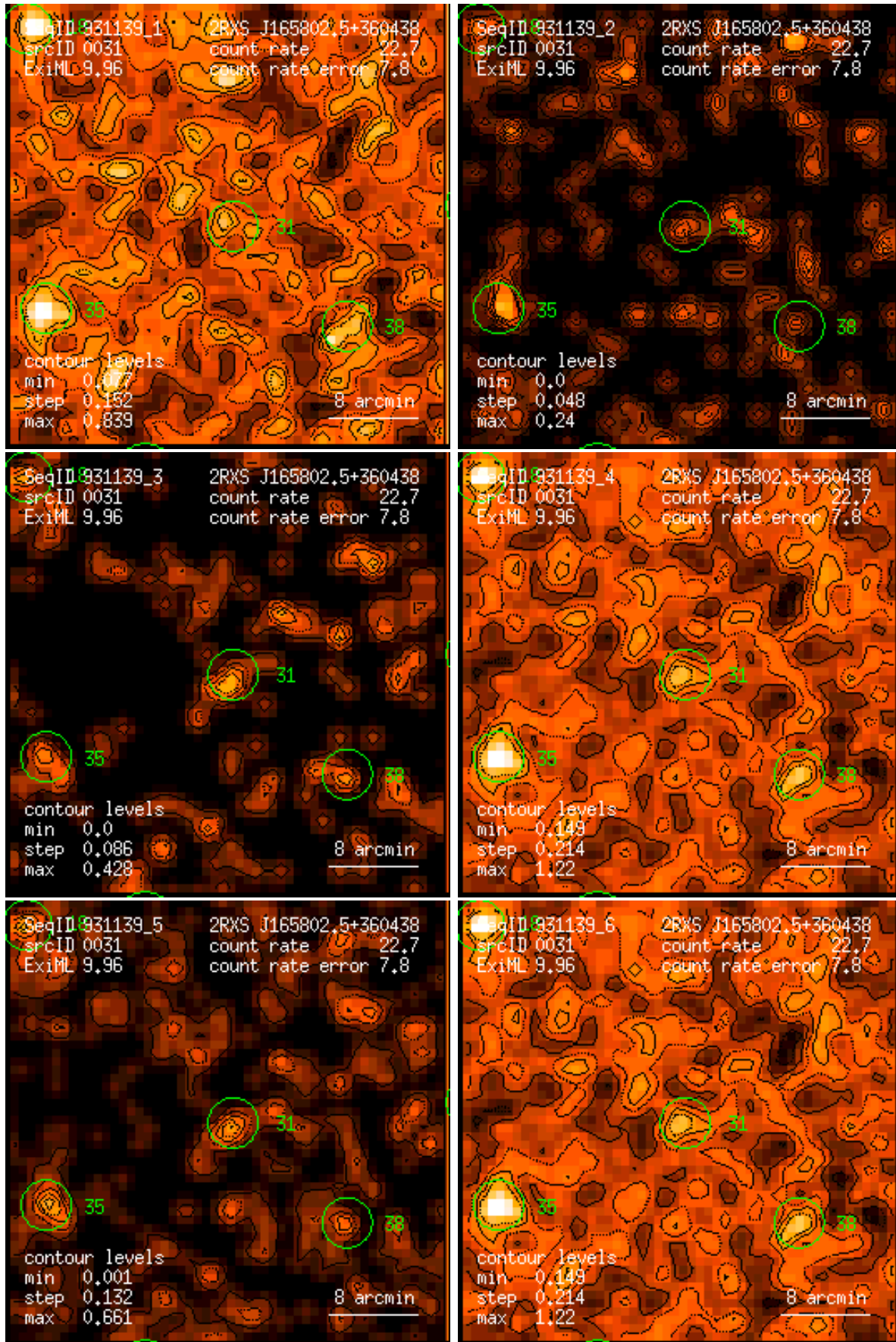
Figure 31: RASS 931139: detection 0031: band rate images, Gaussian filter: (1) PSPC channels 11 – 41, (2) 52 – 90, (3) 91 – 201, (4) 11 – 235, (5) 52 – 201, (6) 11 – 201. Broad band rates in counts/ks. Band rate contour levels in counts/ks/arcmin 2 .
